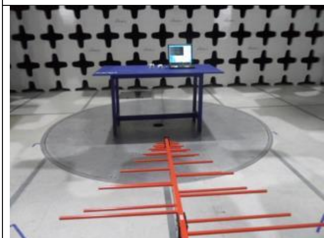
Radiated Emissions (<1GHz) – Front View (Int. Antennas)
