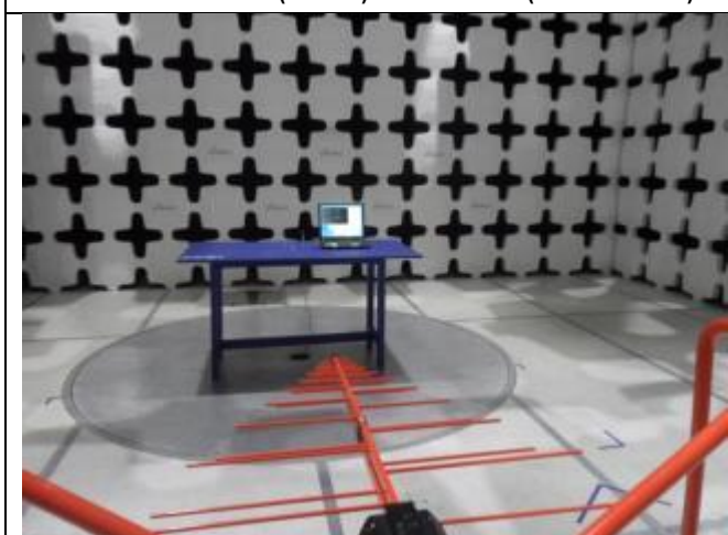
Radiated Emissions (<1GHz) – Front View (Ext. Antennas)
