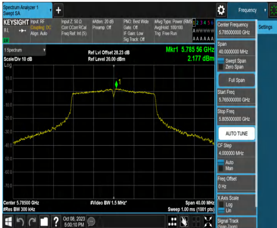
11A-CDD_Ant2_5785
