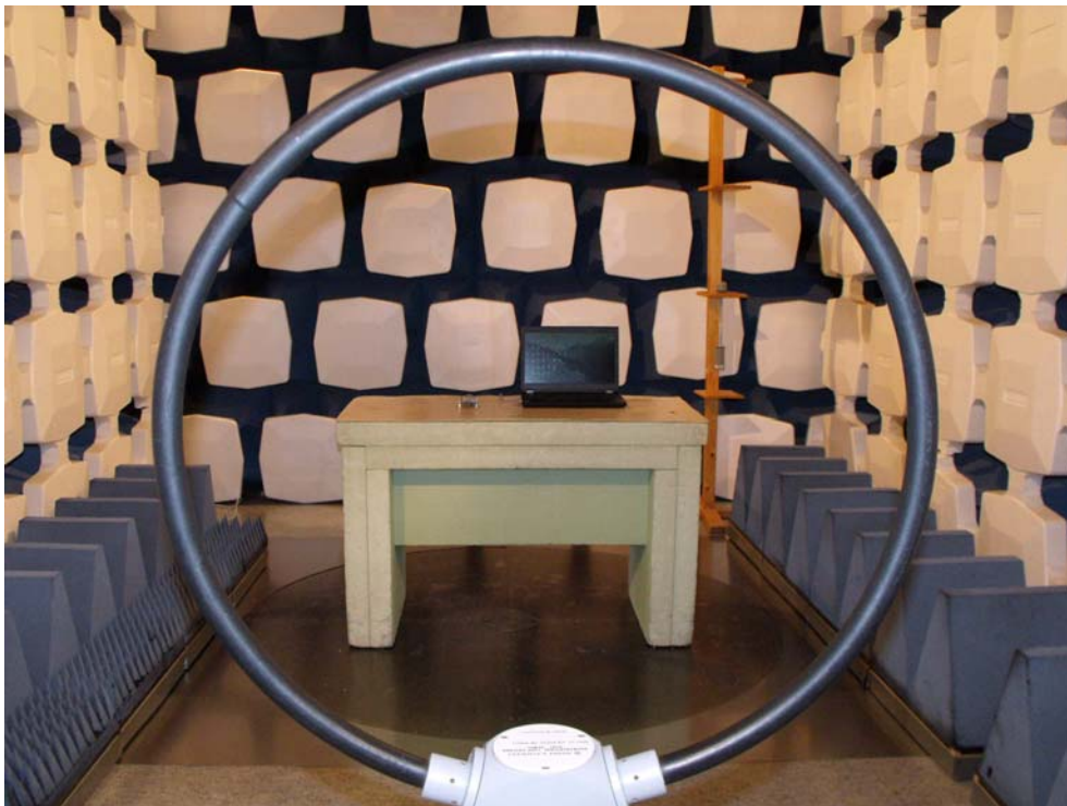
Figure 4: Radiated emission test - SAC
