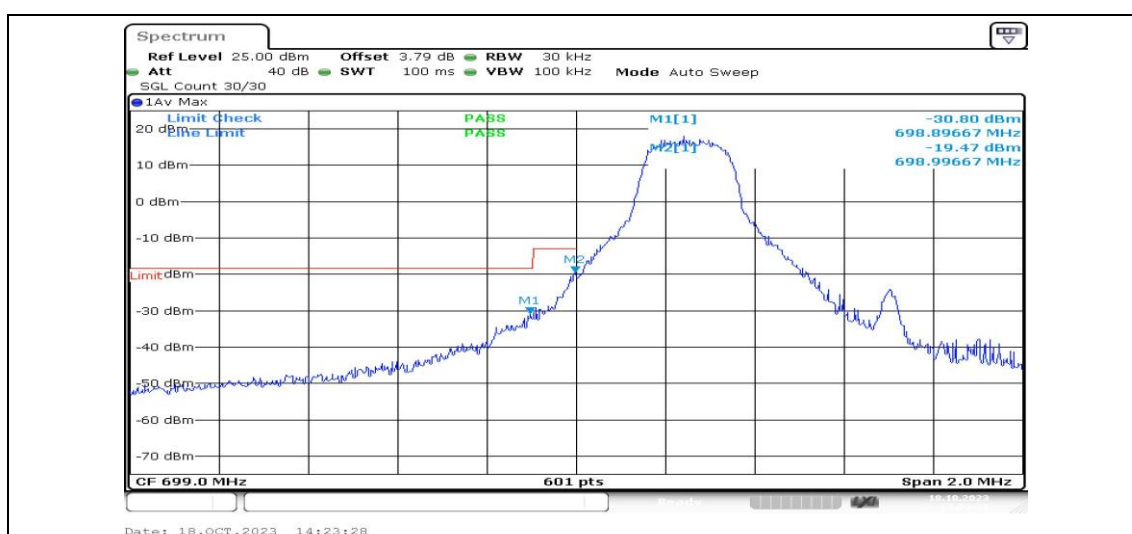
Band12-1.4MHz-QPSK-23017-1RB#0-PASS
