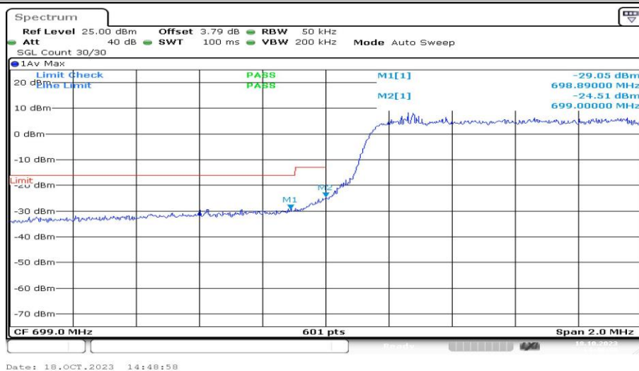
Band12-3MHz-QPSK-23025-15RB#0-PASS
