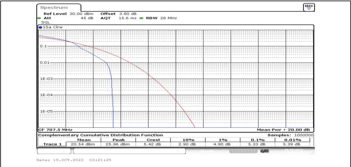
Band12-10MHz-16QAM-23095-1RB#0-PASS
