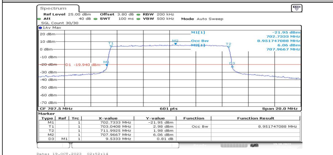
Band12-10MHz-QPSK-23095-50RB#0-PASS
