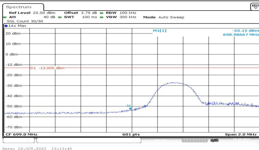
Band12-5MHz-QPSK-23035-1RB#24-PASS
