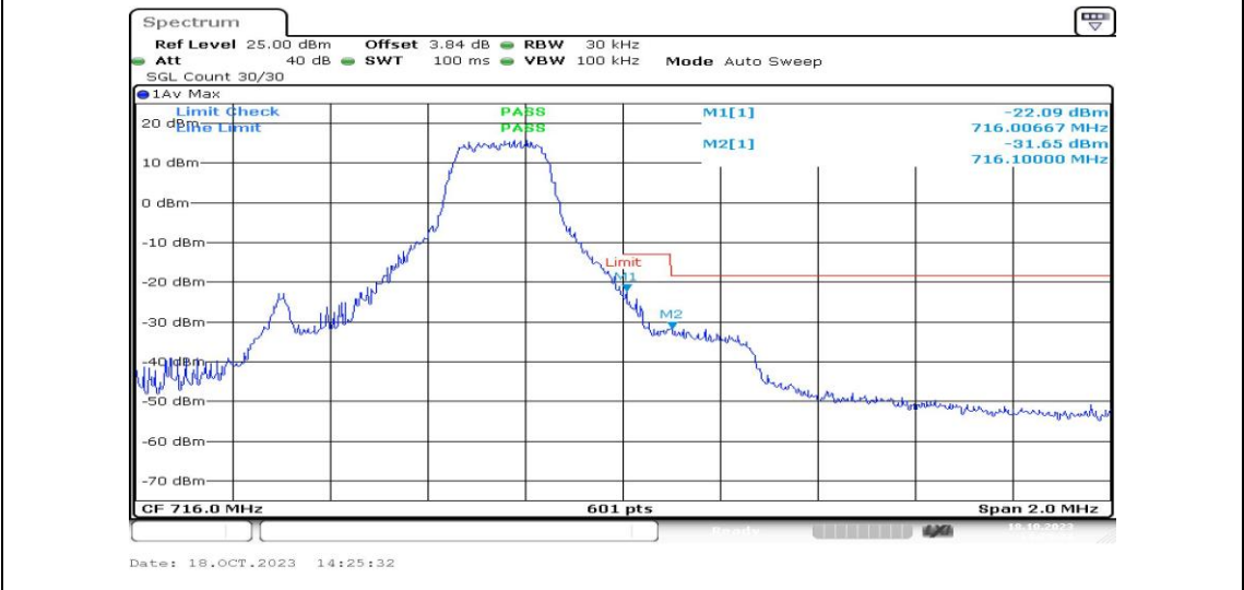
Band12-1.4MHz-16QAM-23173-1RB#5-PASS
