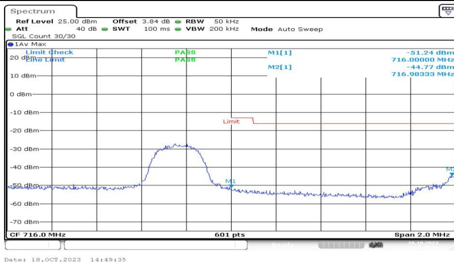
Band12-3MHz-QPSK-23165-1RB#0-PASS
