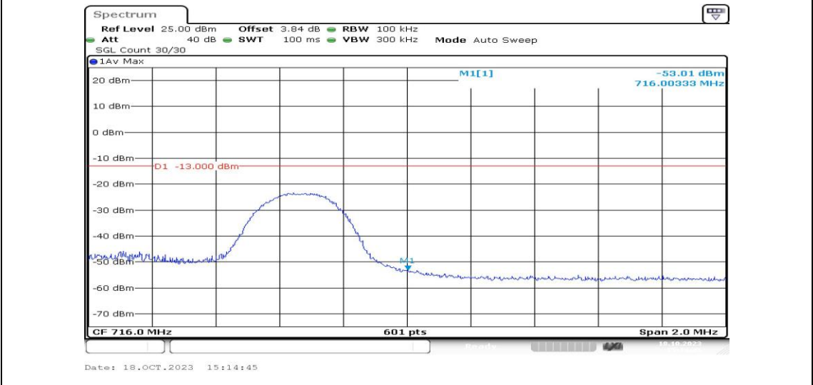
Band12-5MHz-QPSK-23155-1RB#0-PASS
