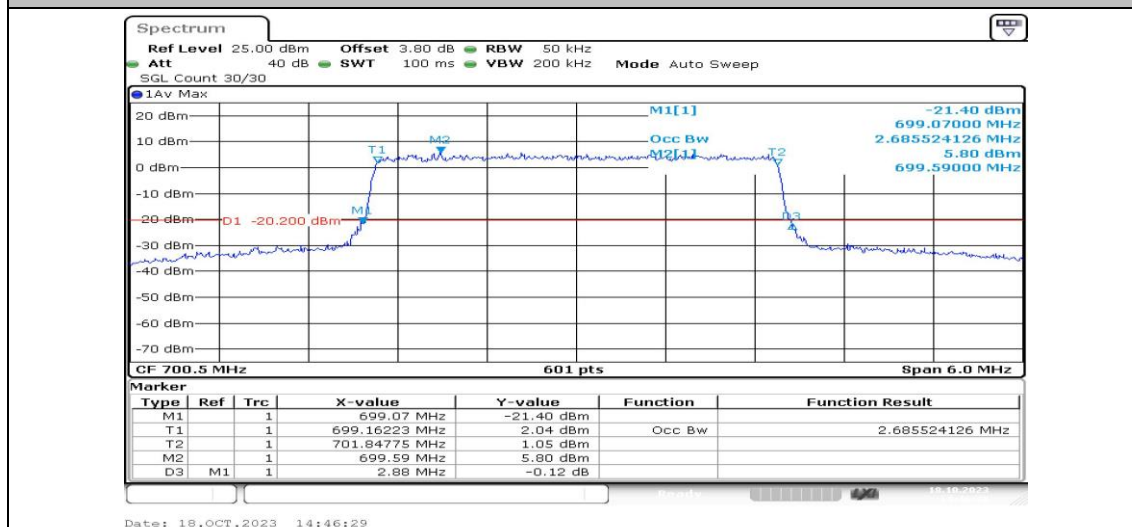
Band12-3MHz-16QAM-23025-15RB#0-PASS
