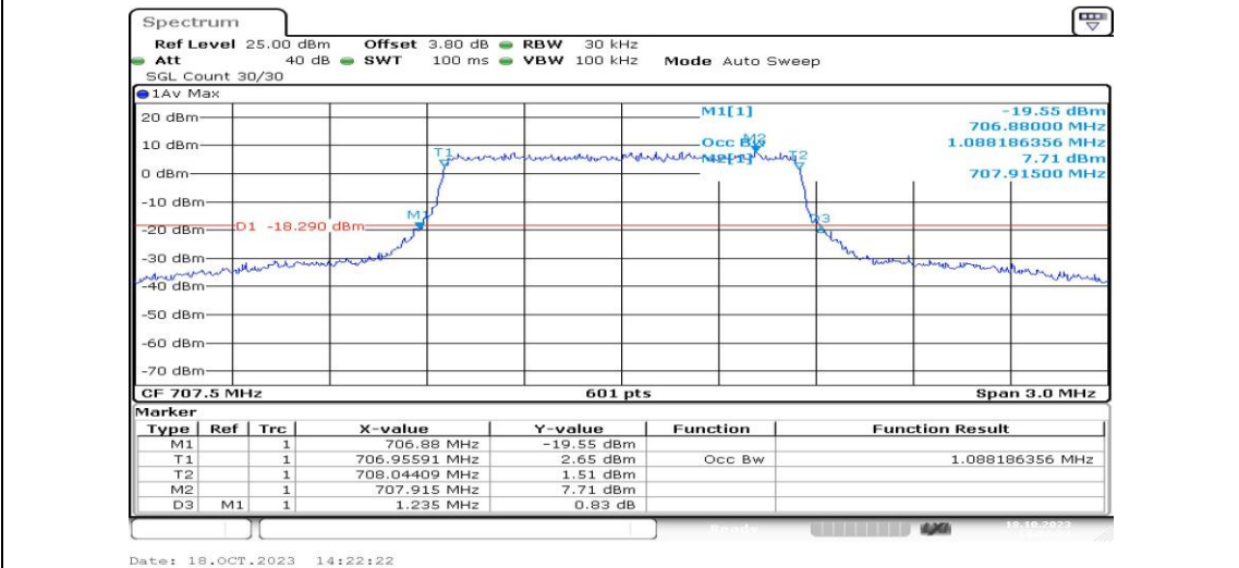
Band12-1.4MHz-16QAM-23095-6RB#0-PASS
