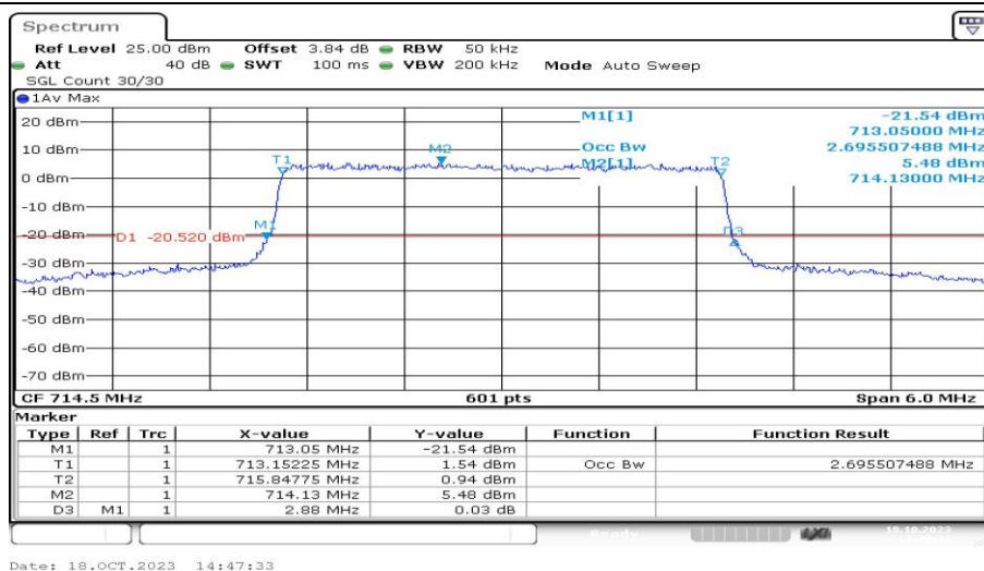
Band12-3MHz-16QAM-23165-15RB#0-PASS
