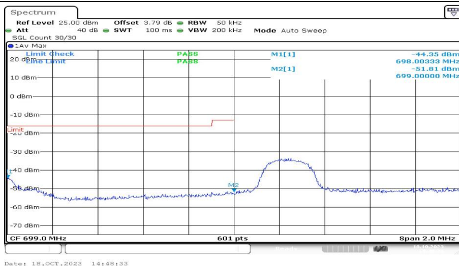
Band12-3MHz-QPSK-23025-1RB#14-PASS
