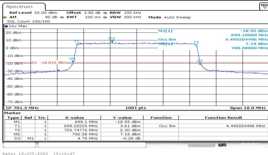
Band12-5MHz-QPSK-23035-25RB#0-PASS
