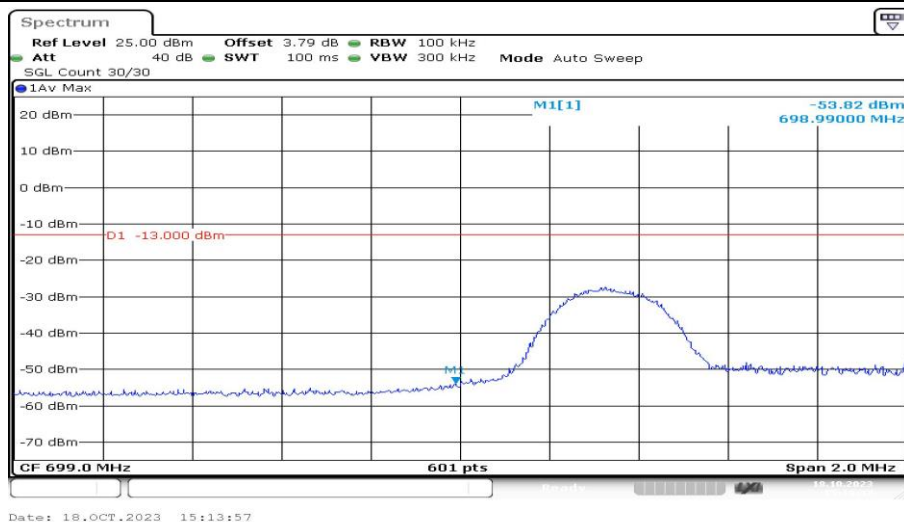
Band12-5MHz-16QAM-23035-1RB#24-PASS
