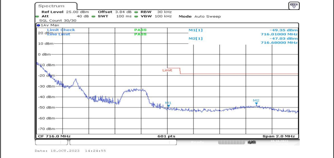
Band12-1.4MHz-QPSK-23173-1RB#0-PASS
