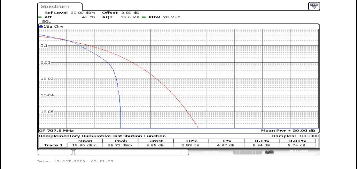
Band12-10MHz-16QAM-23095-25RB#0-PASS
