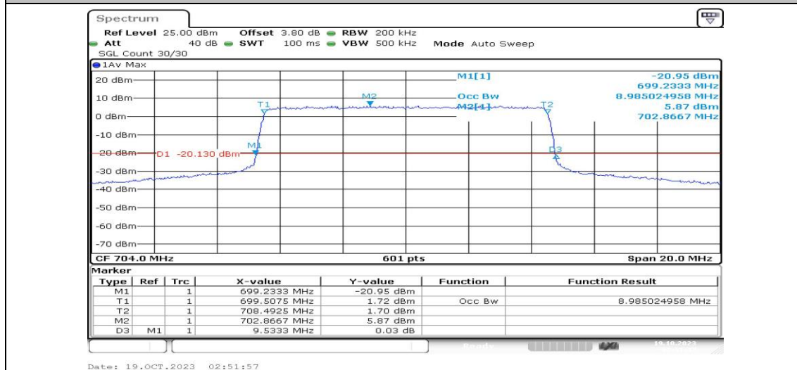
Band12-10MHz-QPSK-23060-50RB#0-PASS
