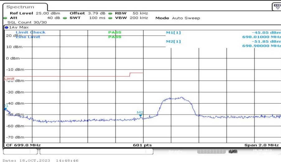
Band12-3MHz-16QAM-23025-1RB#14-PASS
