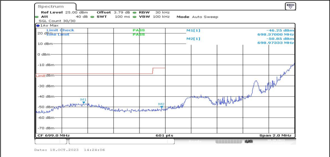
Band12-1.4MHz-16QAM-23017-1RB#5-PASS
