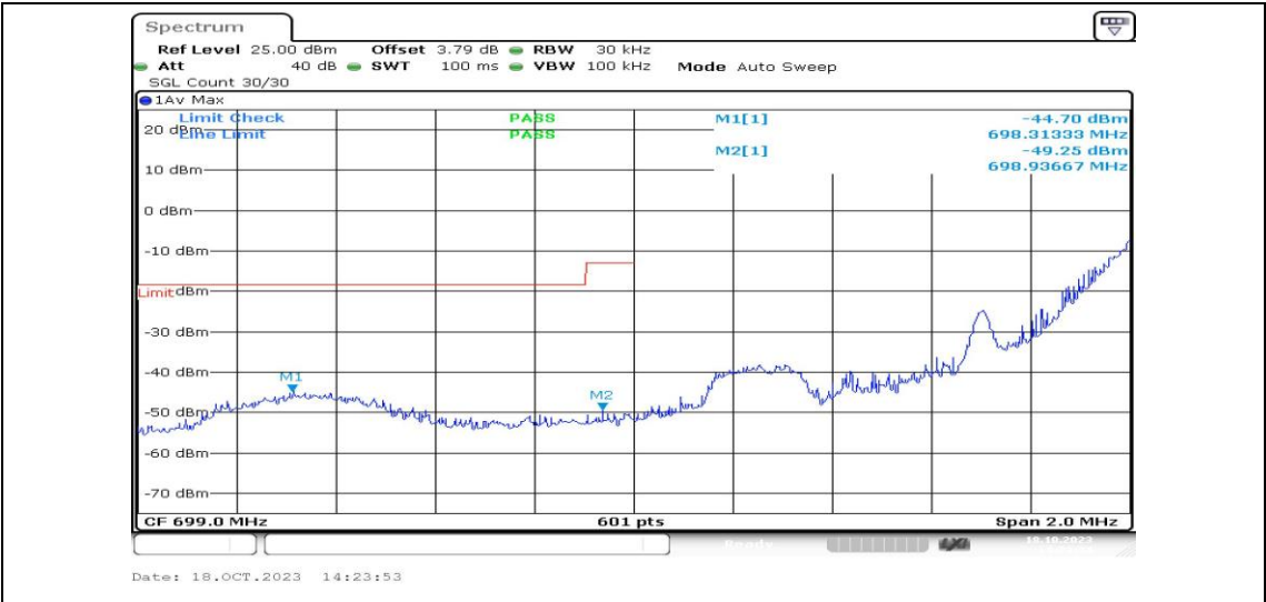
Band12-1.4MHz-QPSK-23017-1RB#5-PASS
