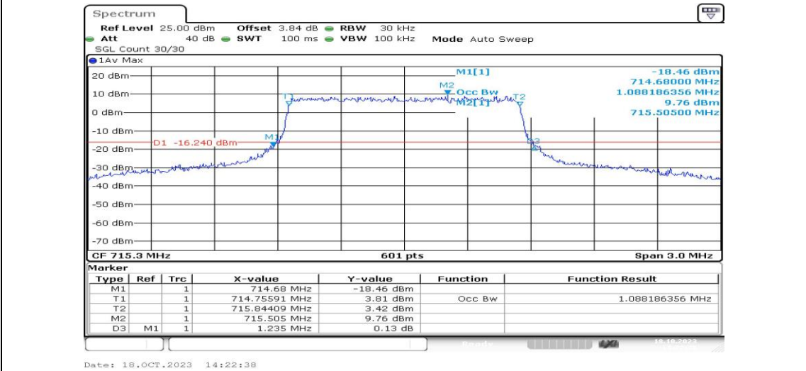
Band12-1.4MHz-QPSK-23173-6RB#0-PASS
