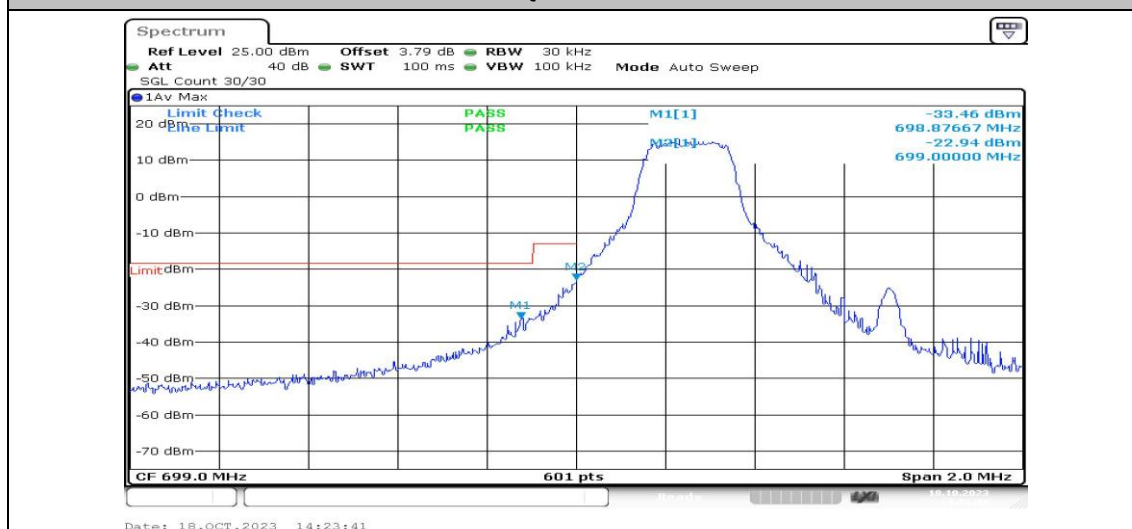
Band12-1.4MHz-16QAM-23017-1RB#0-PASS
