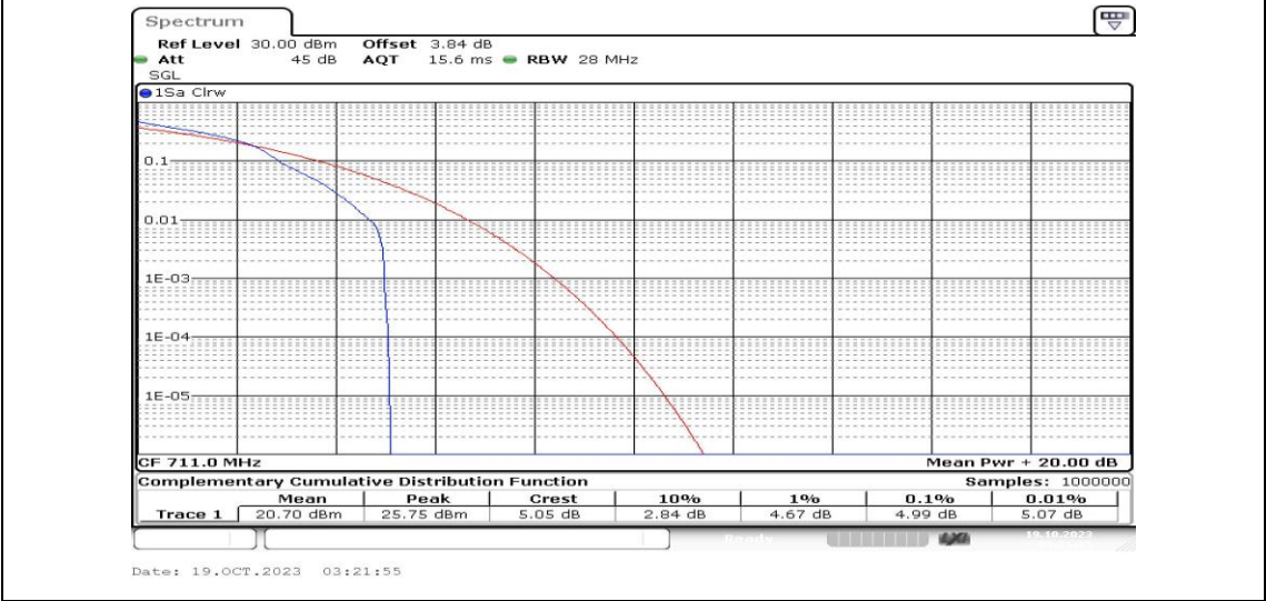
Band12-10MHz-16QAM-23130-1RB#0-PASS
