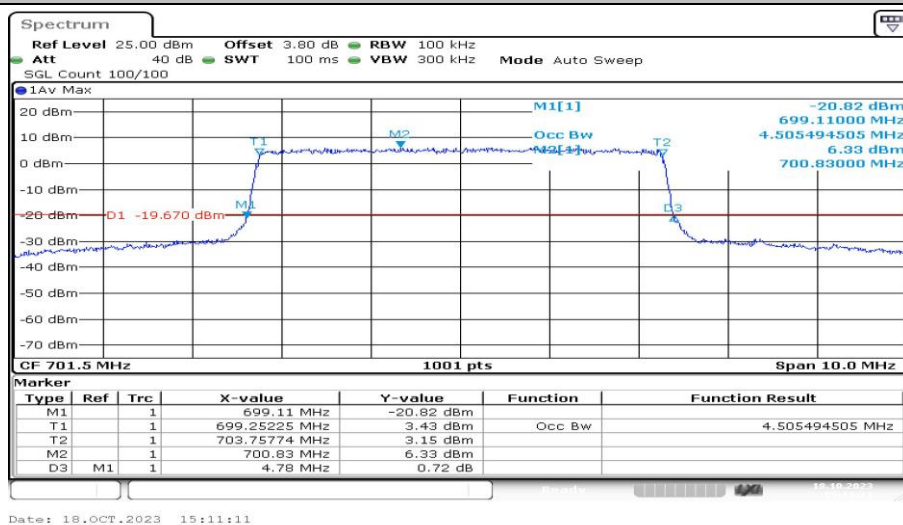
Band12-5MHz-16QAM-23035-25RB#0-PASS
