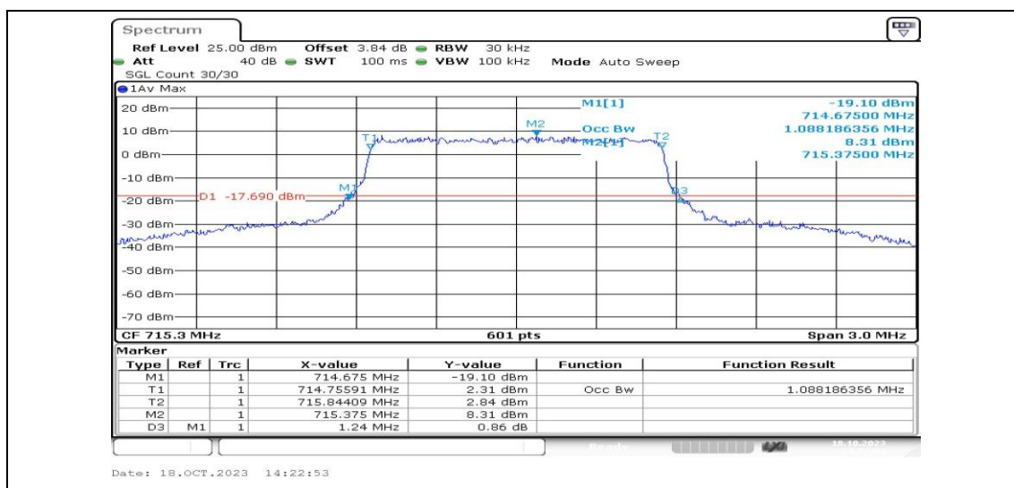
Band12-1.4MHz-16QAM-23173-6RB#0-PASS
