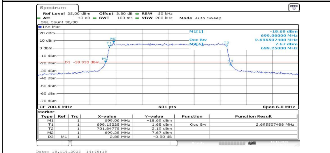
Band12-3MHz-QPSK-23025-15RB#0-PASS
