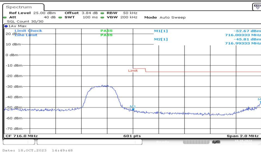
Band12-3MHz-16QAM-23165-1RB#0-PASS
