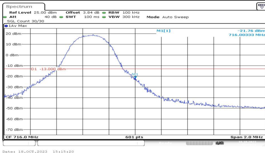
Band12-5MHz-16QAM-23155-1RB#24-PASS
