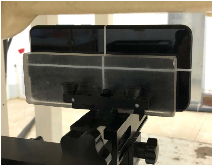
Right Side (Test distance: 10mm)
