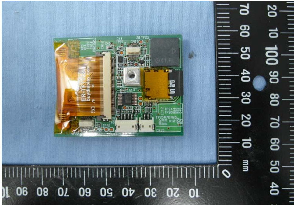
EUT Photo (42)
