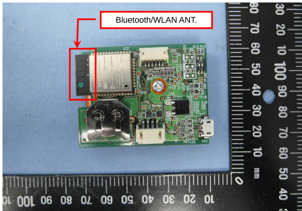
EUT Photo (32)
