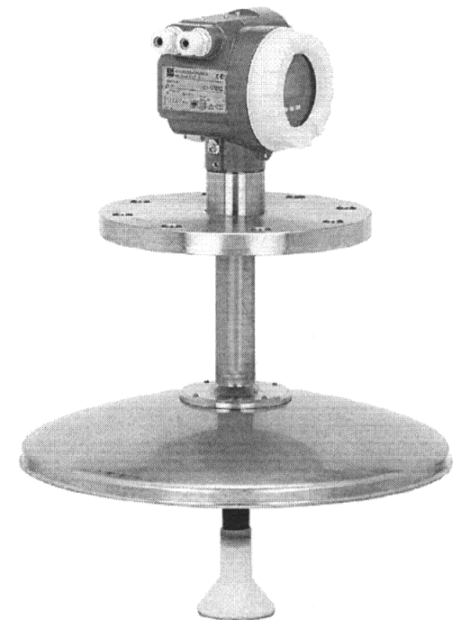
FMR 533 Parabolantenne Parabolic antenna
