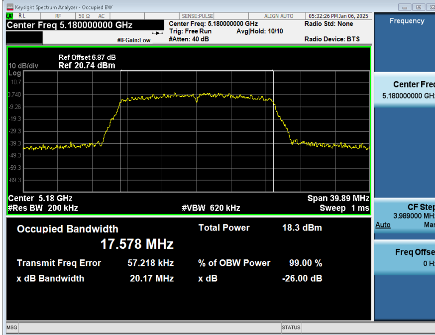
99%_OCB_NVNT_ANT2_802_11n(HT20)_5180
