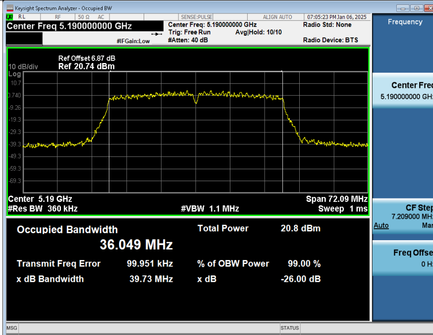
-26BW_NVNT_ANT2_802_11n(HT40)_5190
