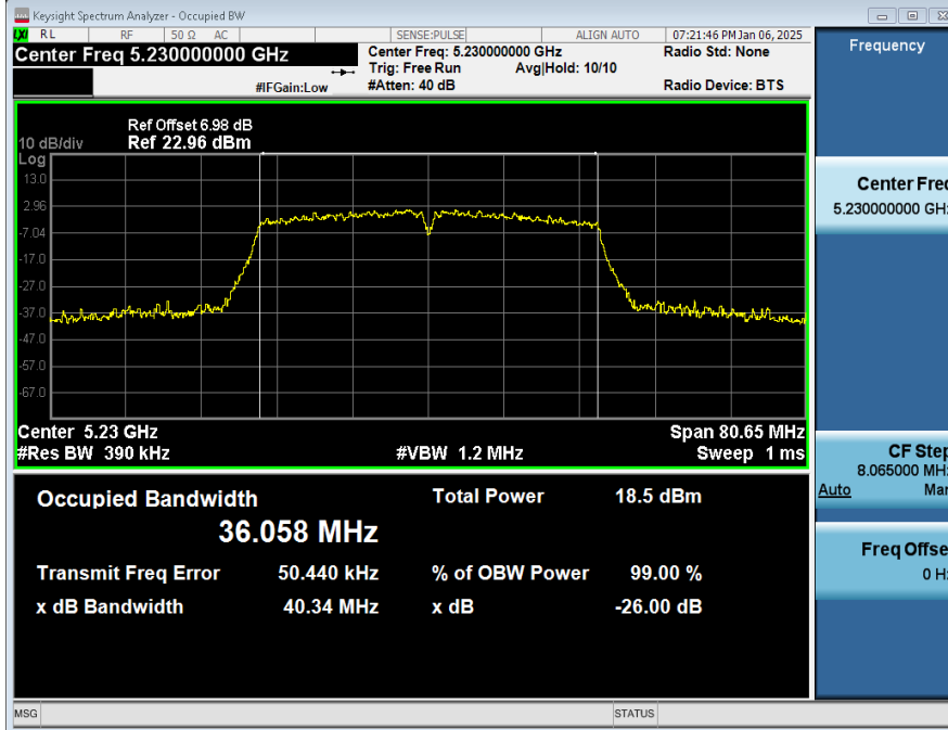
99%_OCB_NVNT_ANT2_802_11ac(VHT40)_5230
