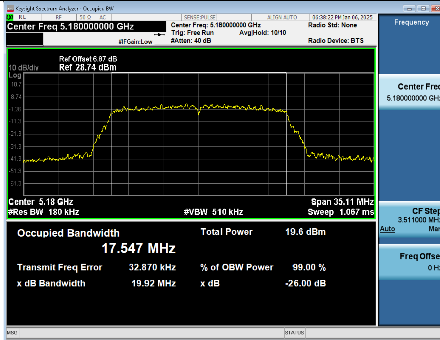
-26BW_NVNT_ANT2_802_11ac(VHT20)_5180
