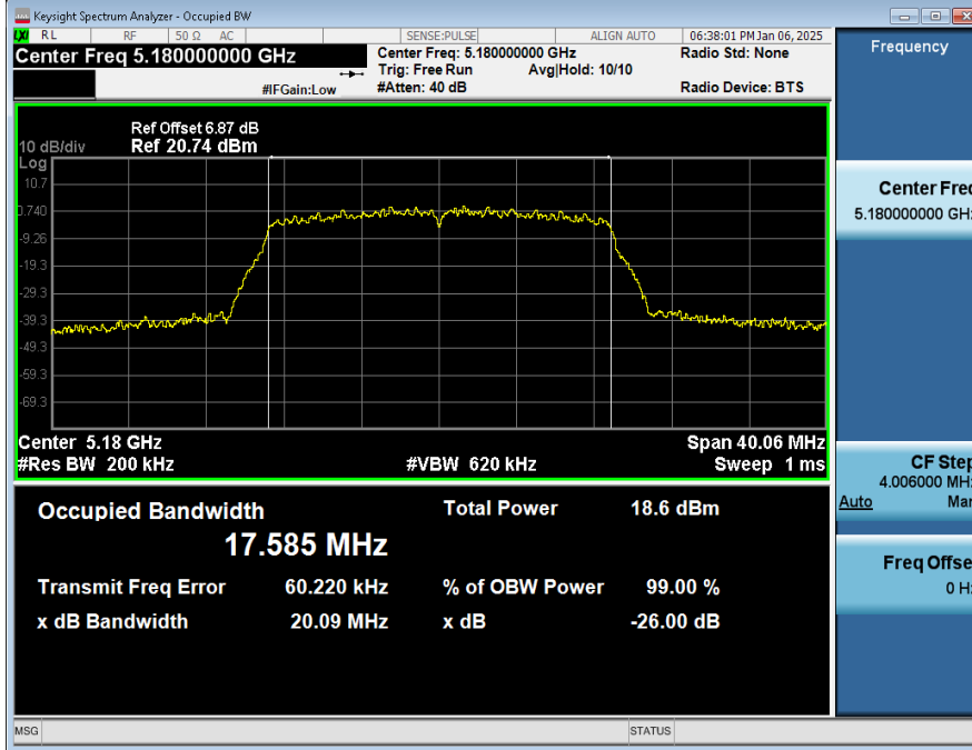
99%_OCB_NVNT_ANT2_802_11ac(VHT20)_5180
