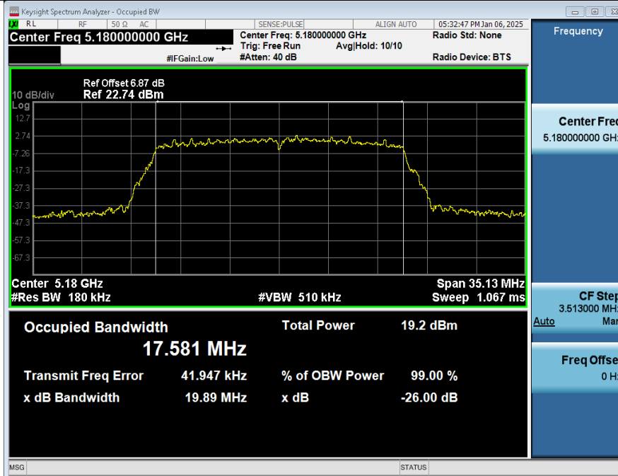
-26BW_NVNT_ANT2_802_11n(HT20)_5180
