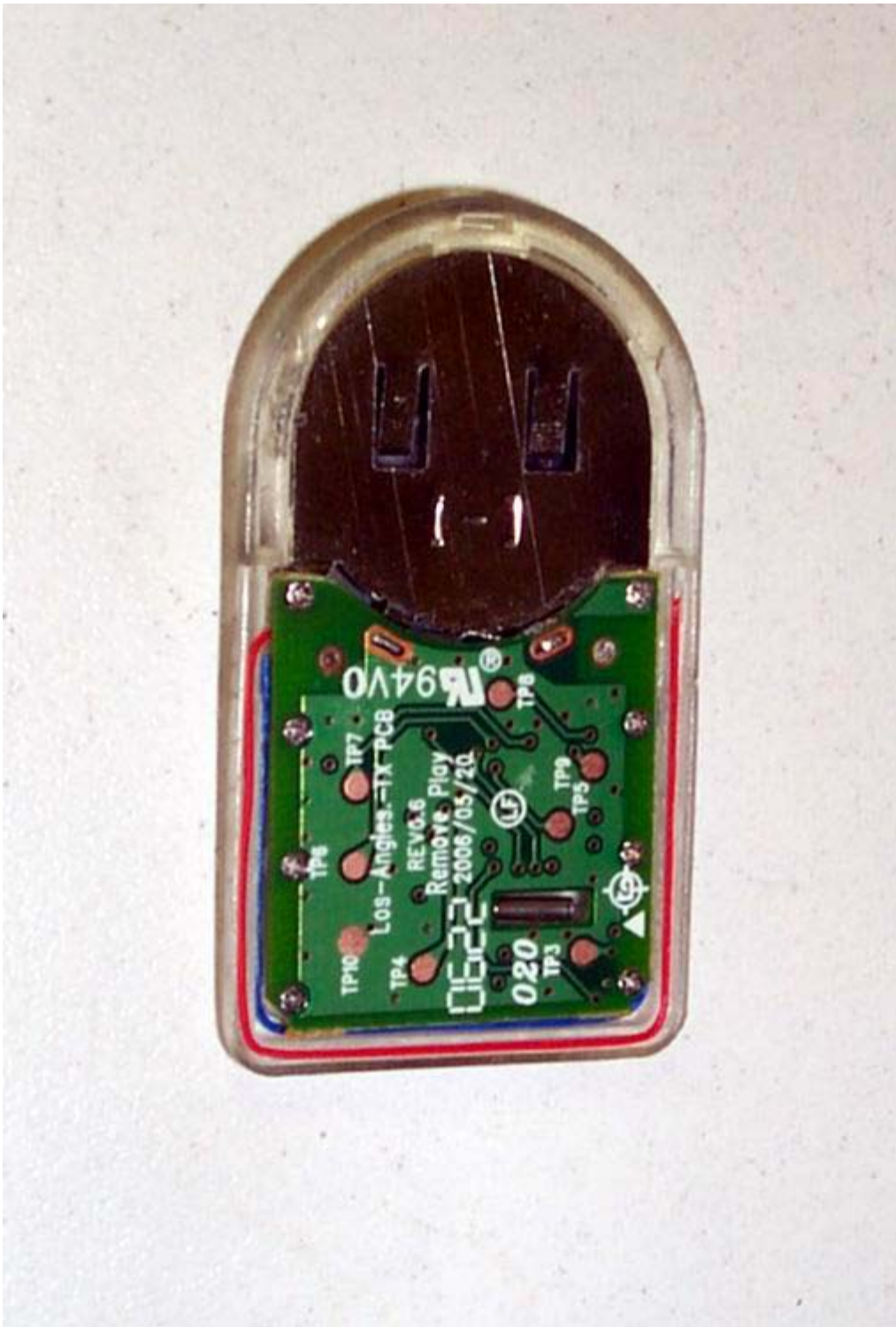
Back View-TA-100
