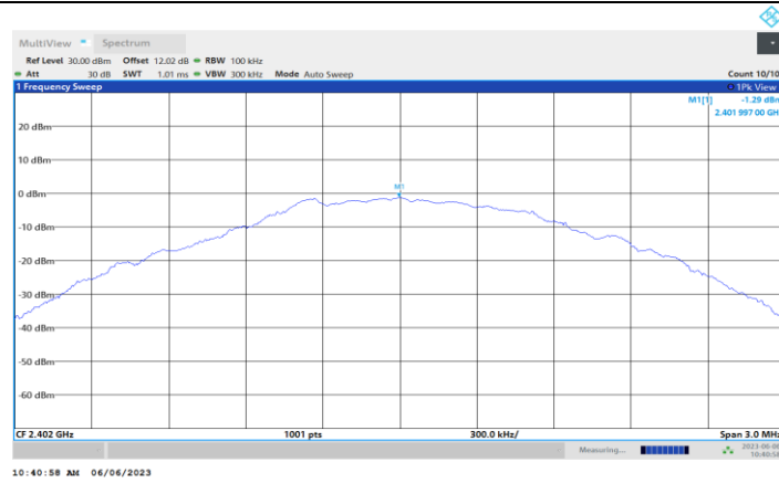
BLE_2M_Ant1_2402_0~Reference
