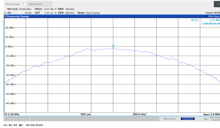
BLE_2M_Ant1_2440_0~Reference
