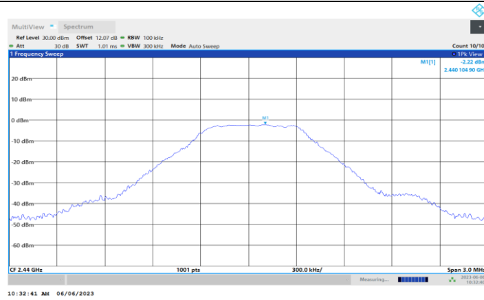
BLE_1M_Ant1_2440_0~Reference
