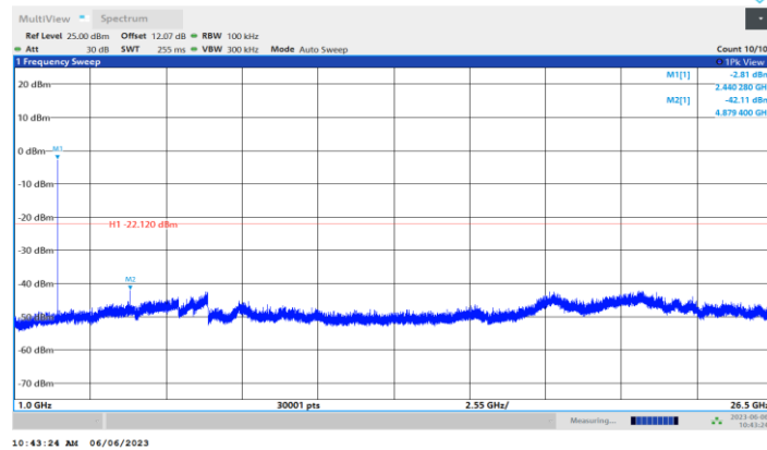
BLE_2M_Ant1_2440_1000~26500
