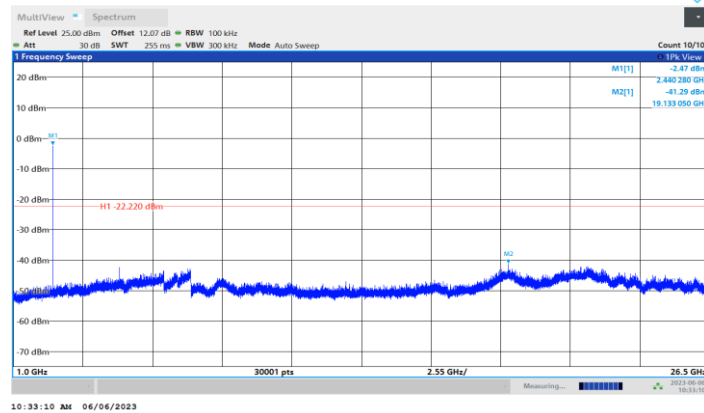
BLE_1M_Ant1_2440_1000~26500
