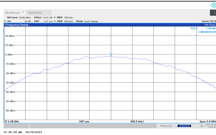
BLE_2M_Ant1_2480_0~Reference
