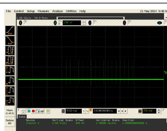
Radar Pulse 0: 18 Pulses
