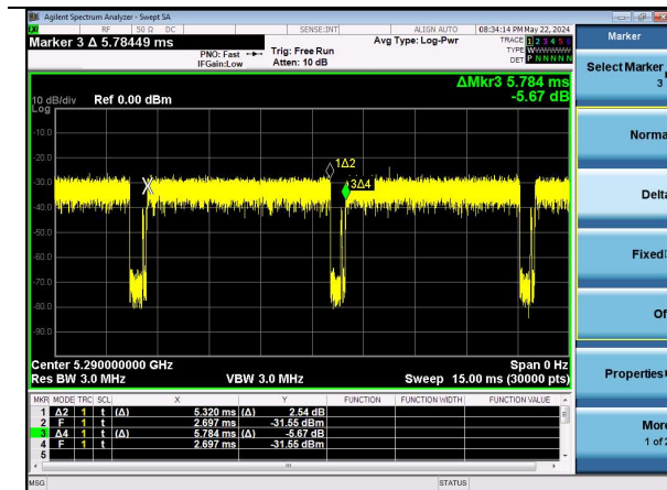
Duty Cycle of iPerf Traffic: 92%
