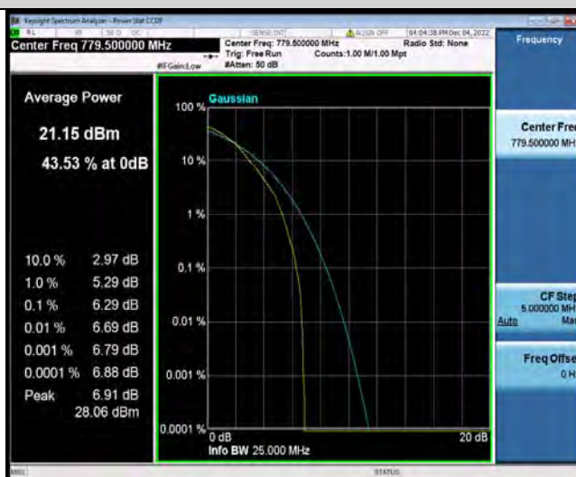
Band13-5MHz-64QAM-23205-25RB#0
