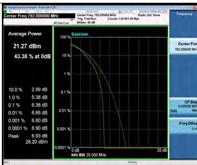
Band13-5MHz-64QAM-23230-25RB#0
