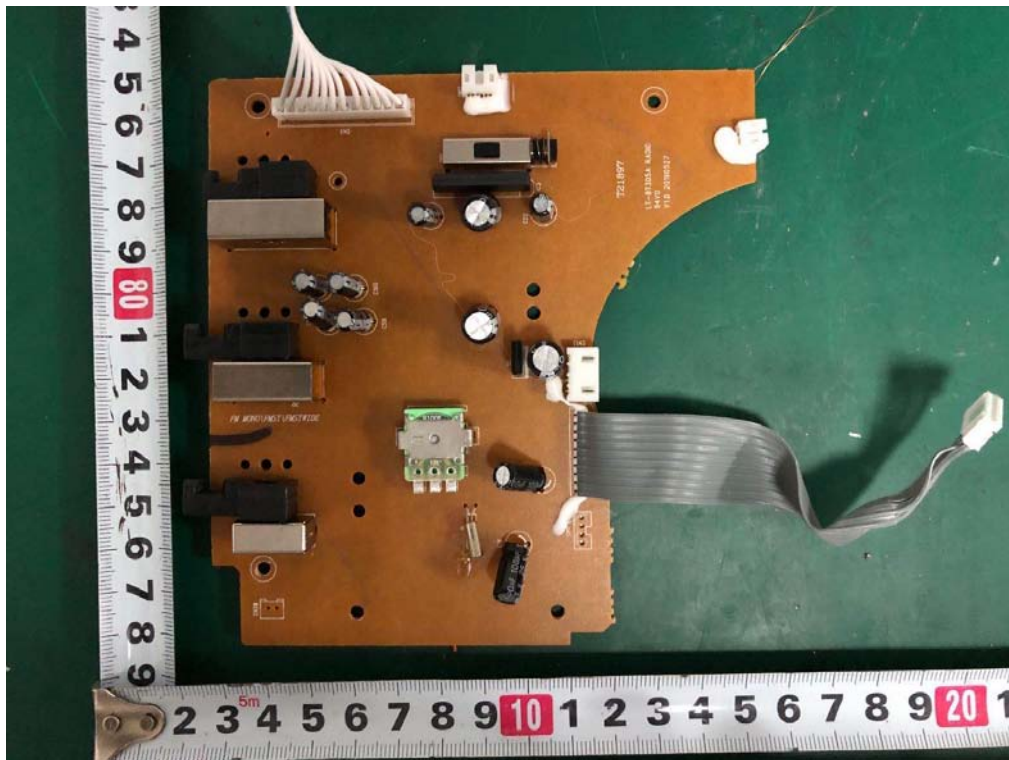
Internal photos M/N: CT201A-BK
