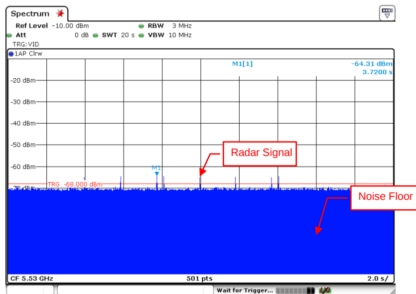
Single Burst of Radar Signal 4
