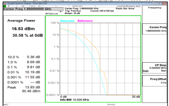
Cat M1 LTE_Band2_10MHz_16QAM_6_0_MidCH18900-1880
