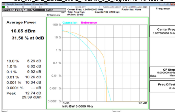
Cat M1 LTE_Band2_5MHz_16QAM_6_0_HighCH19175-1907.5
