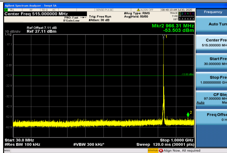
Band5-3MHz-16QAM-20525-1RB#0-30~1000MHz
