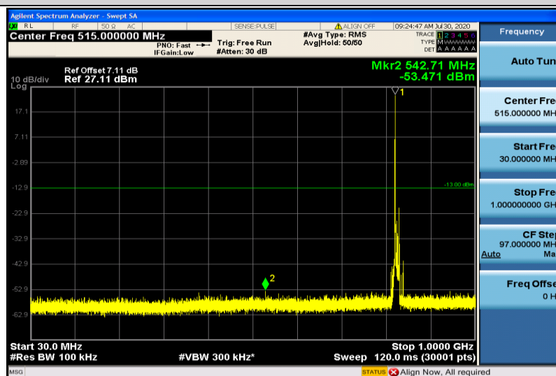
Band5-10MHz-QPSK-20450-1RB#0-30~1000MHz
