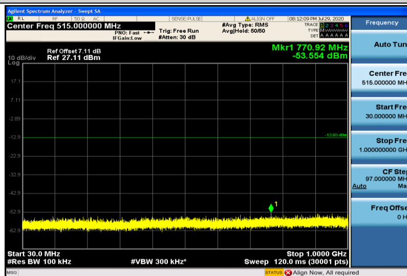
Band4-10MHz-QPSK-20175-1RB#0-30~1000MHz
