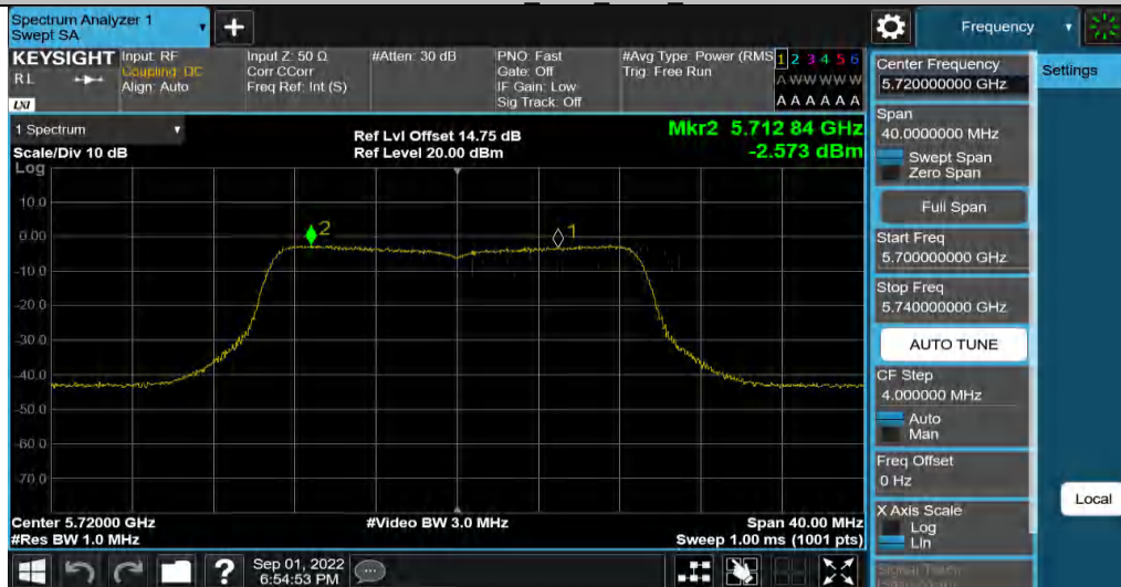
11AC20MIMO_Ant4_5720_UNII-2C
