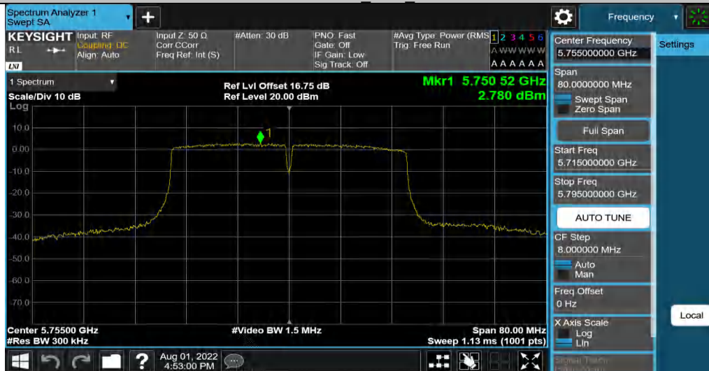
11N40MIMO Ant3 5755
