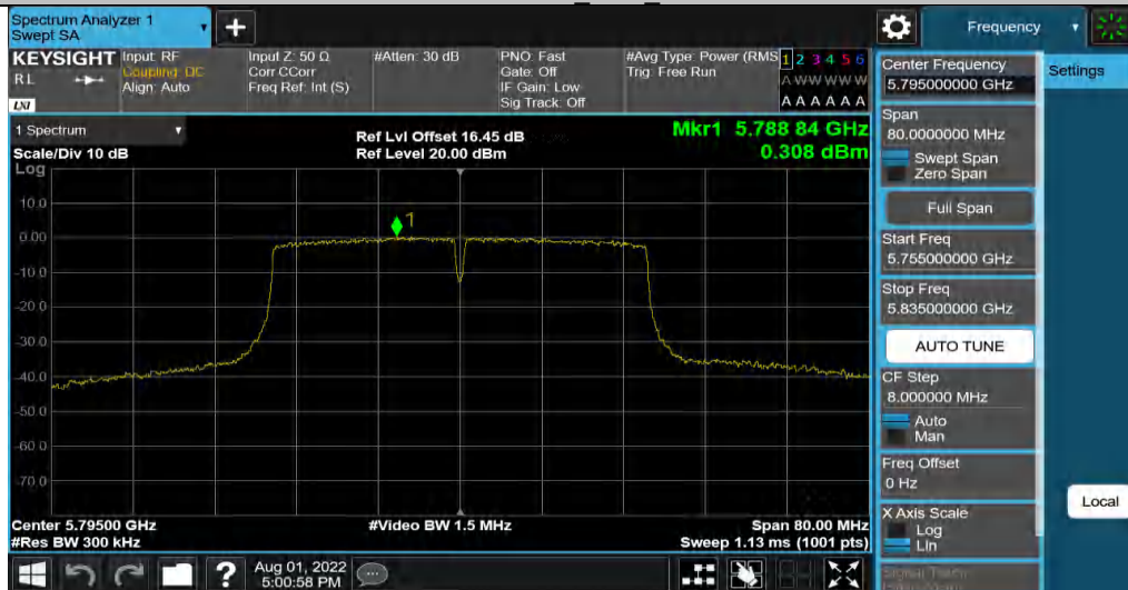
11N40MIMO Ant2 5795
