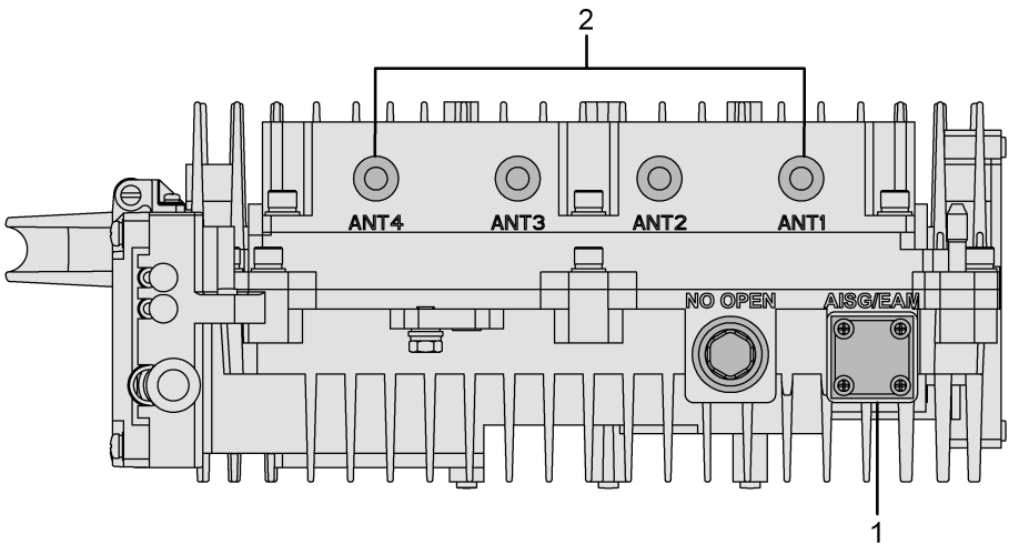
Figure 4-1 External Interfaces 1
