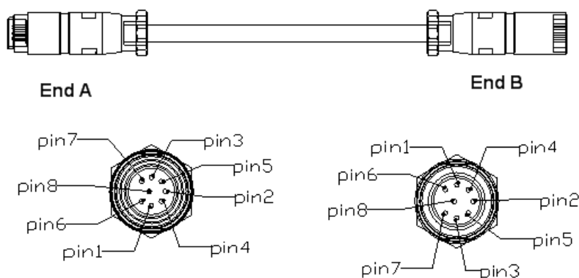
Figure 4-8 AISG Cable
