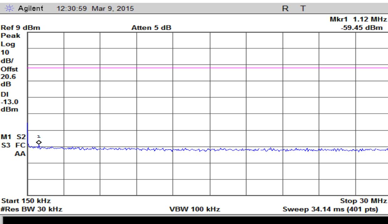
Plot 13 – High Band – 150kHz to 30MHz
