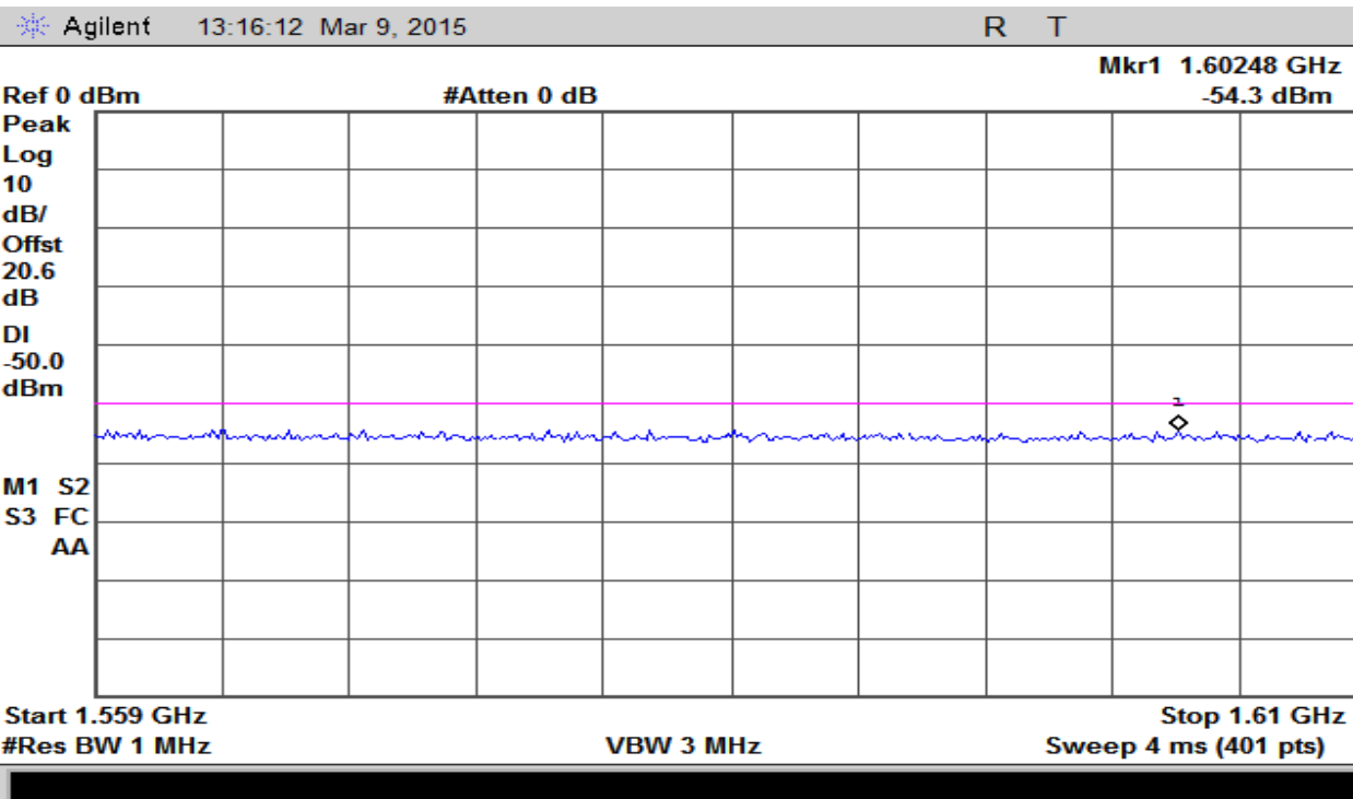
Plot 27- Low Channel - Carrier Off
