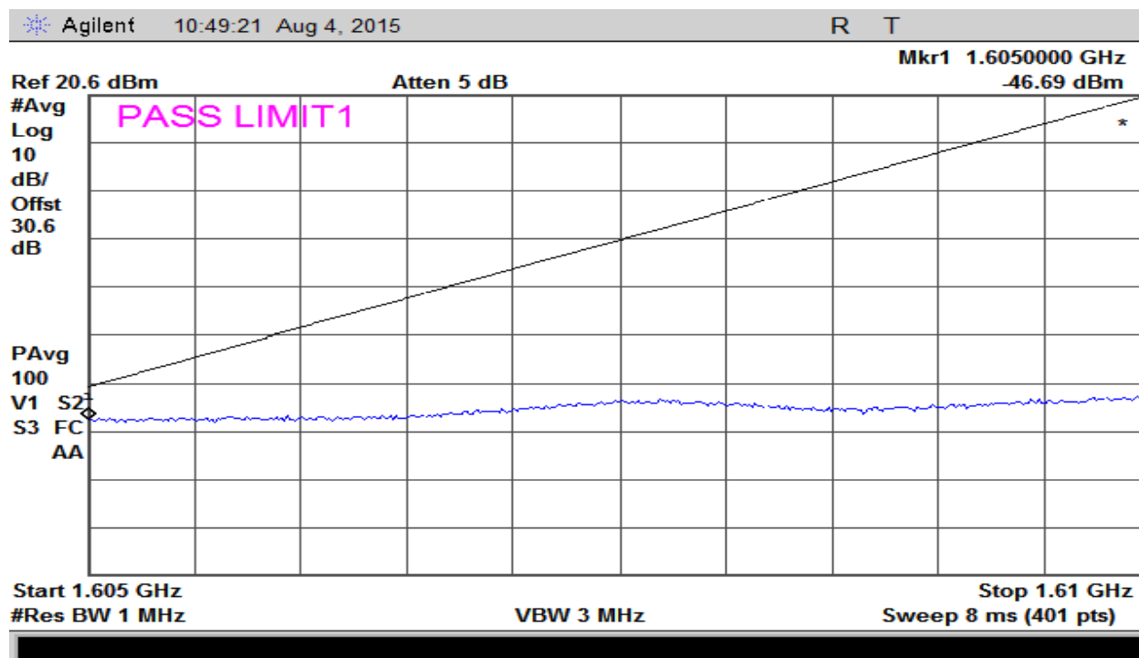
Plot 26-High Channel – Test Limit 25.216 (f)(g)
