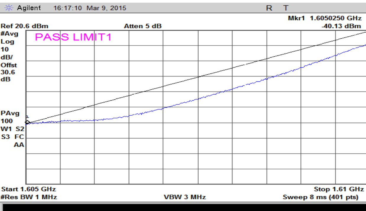
Plot 25- Low Channel – Test Limit 25.216 (f)(g)
