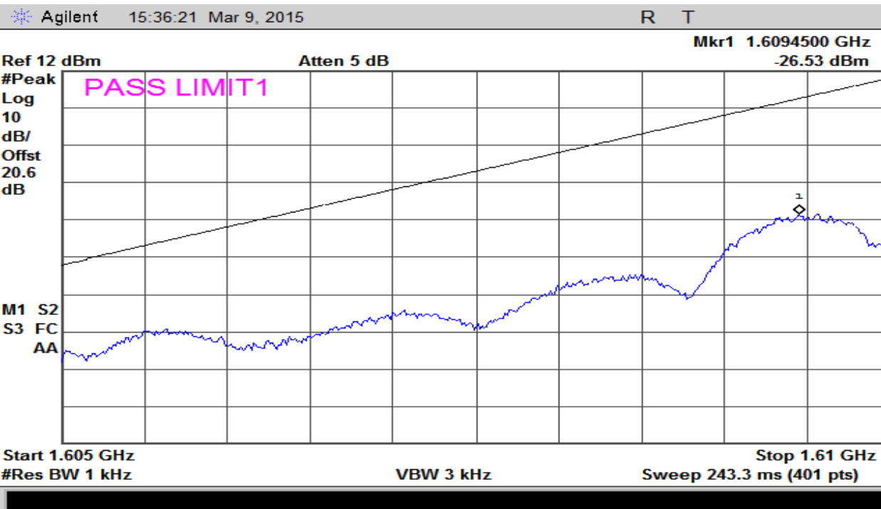
Plot 23- Low Channel – Test Limit 25.216 (f)(g) – Discrete Emissions
