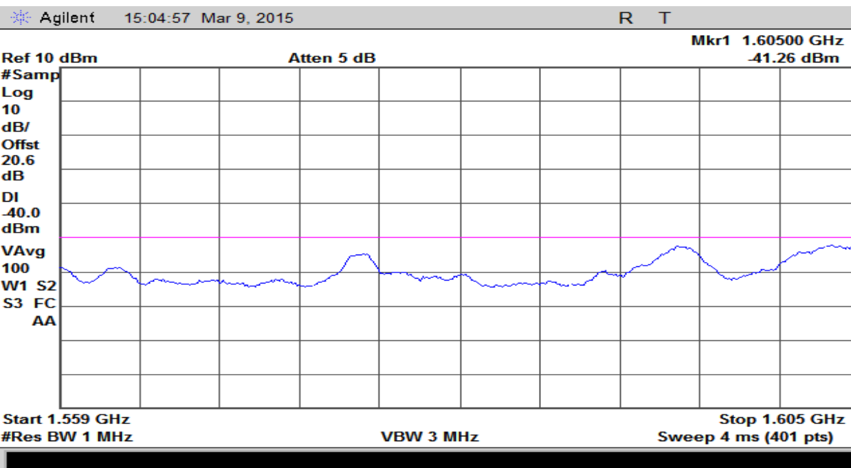
Plot 21 – Low Channel – Test Limit 25.216 (c)
