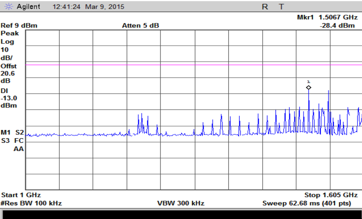
Plot 15 – High Band – 1GHz to 1.605GHz
