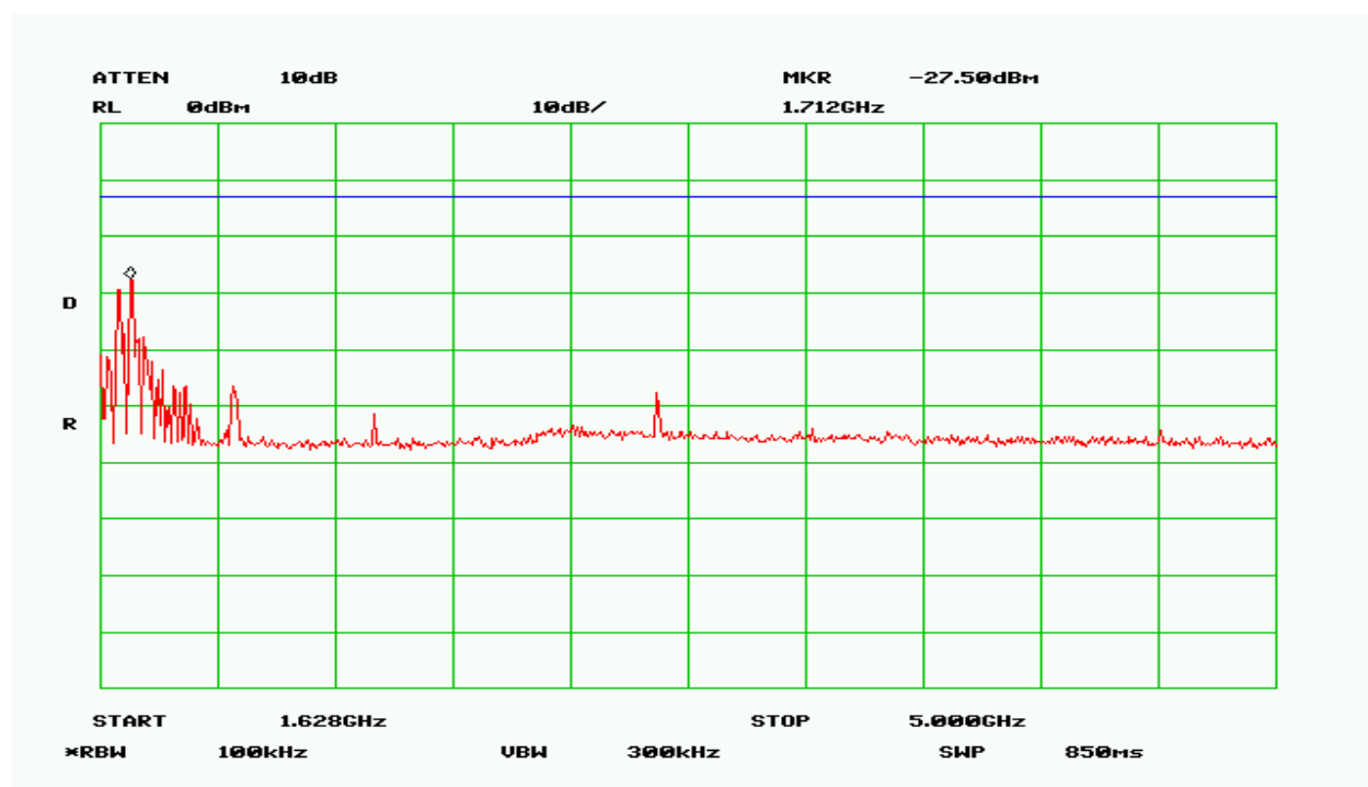
Plot 10 – Low Channel - 1.628 – 5 GHz
