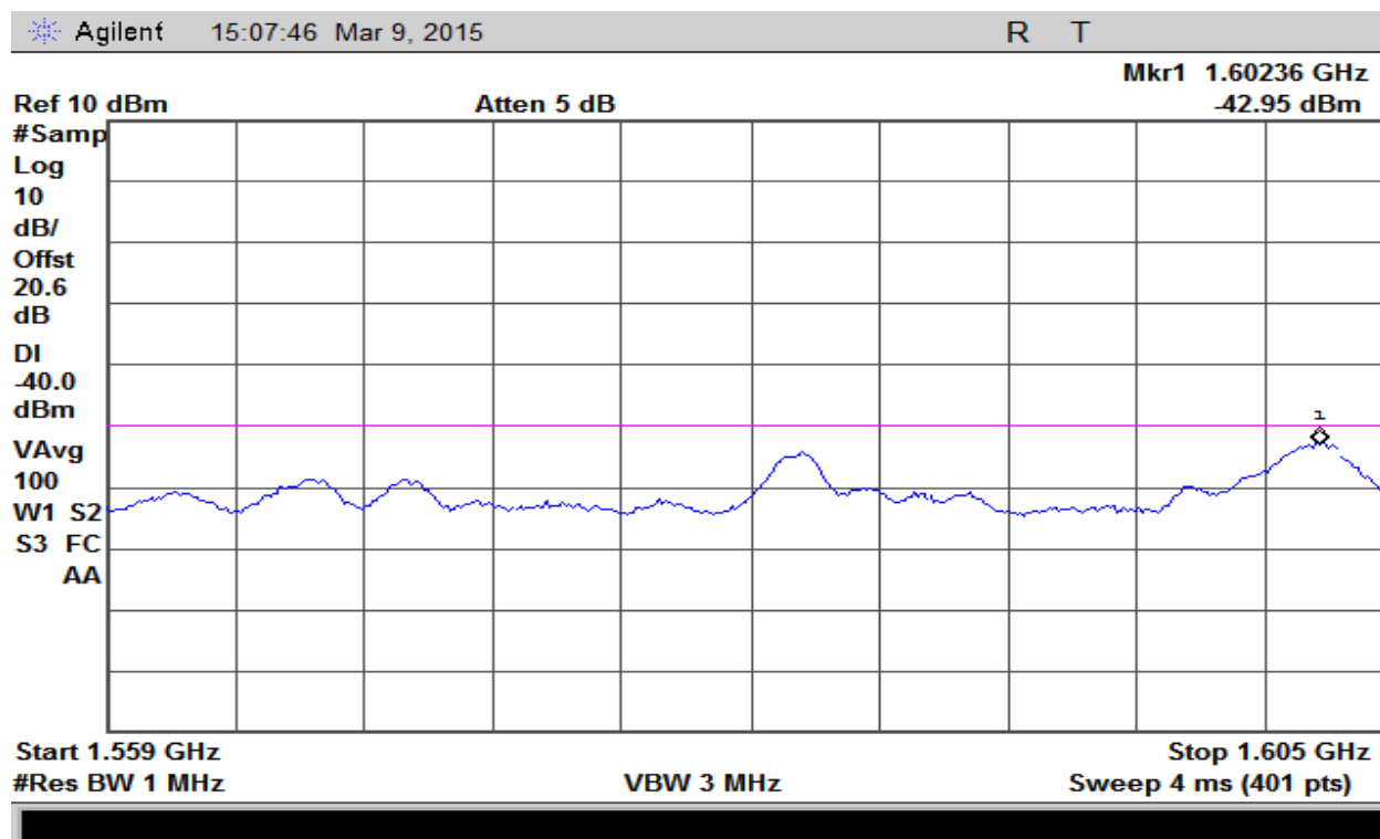
Plot 22 – High Channel – Test Limit 25.216 (c)
