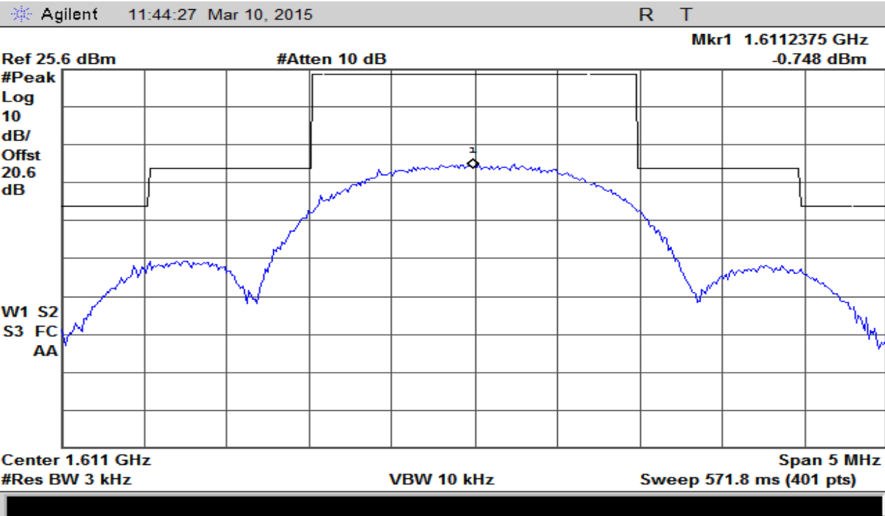
Plot 5 – Low Channel
