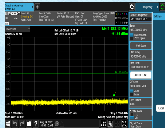
11G-Ant1-2437-30-1000
