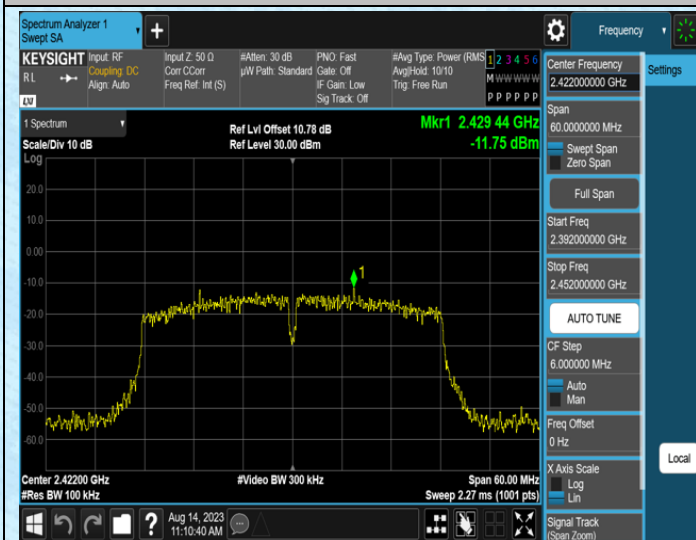
11N40SISO-Ant1-2422-0~Reference
