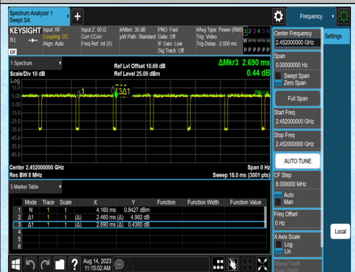
NTNV-11N40SISO-Ant1-2452
