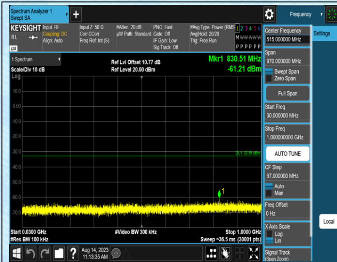
11N40SISO-Ant1-2437-30~1000
