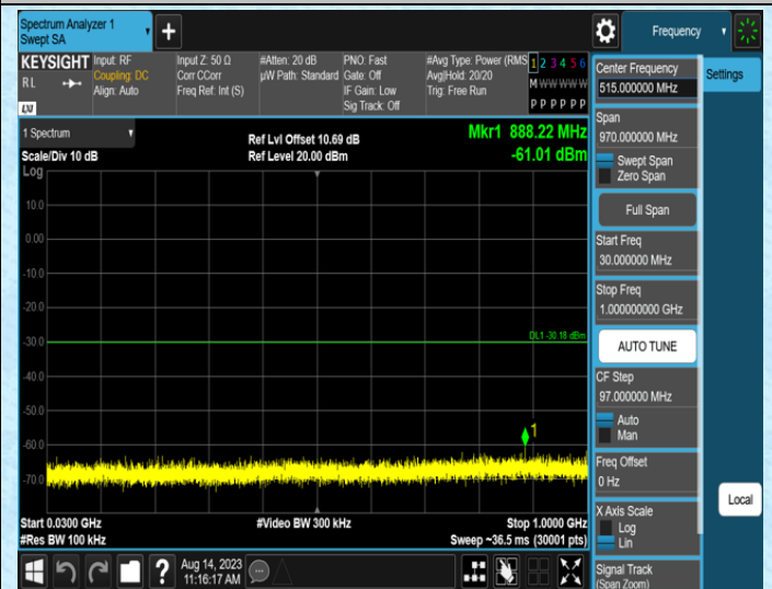
11N40SISO-Ant1-2452-30~1000
