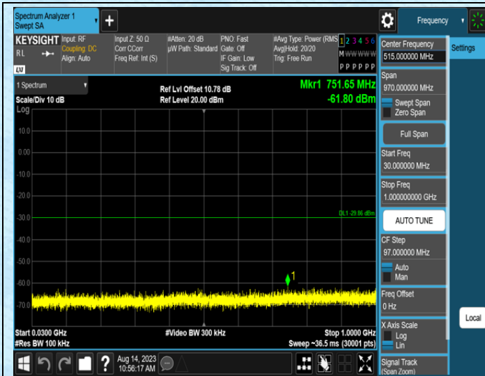
11N20SISO-Ant1-2412-30~1000
