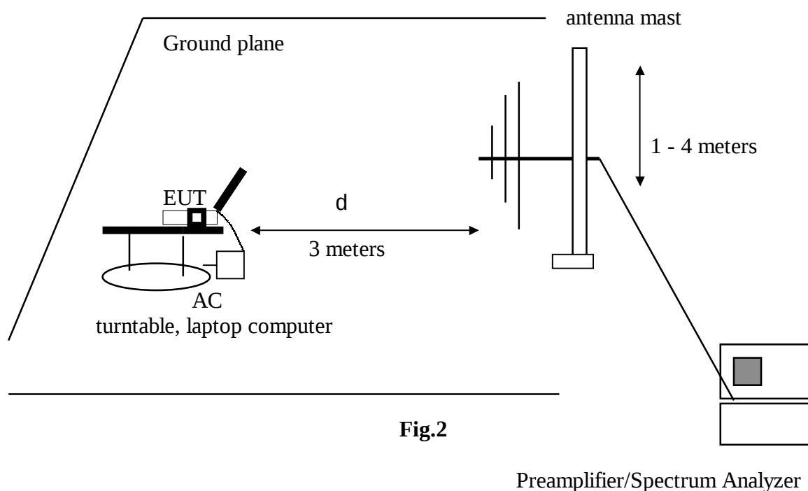
Test Set-up
