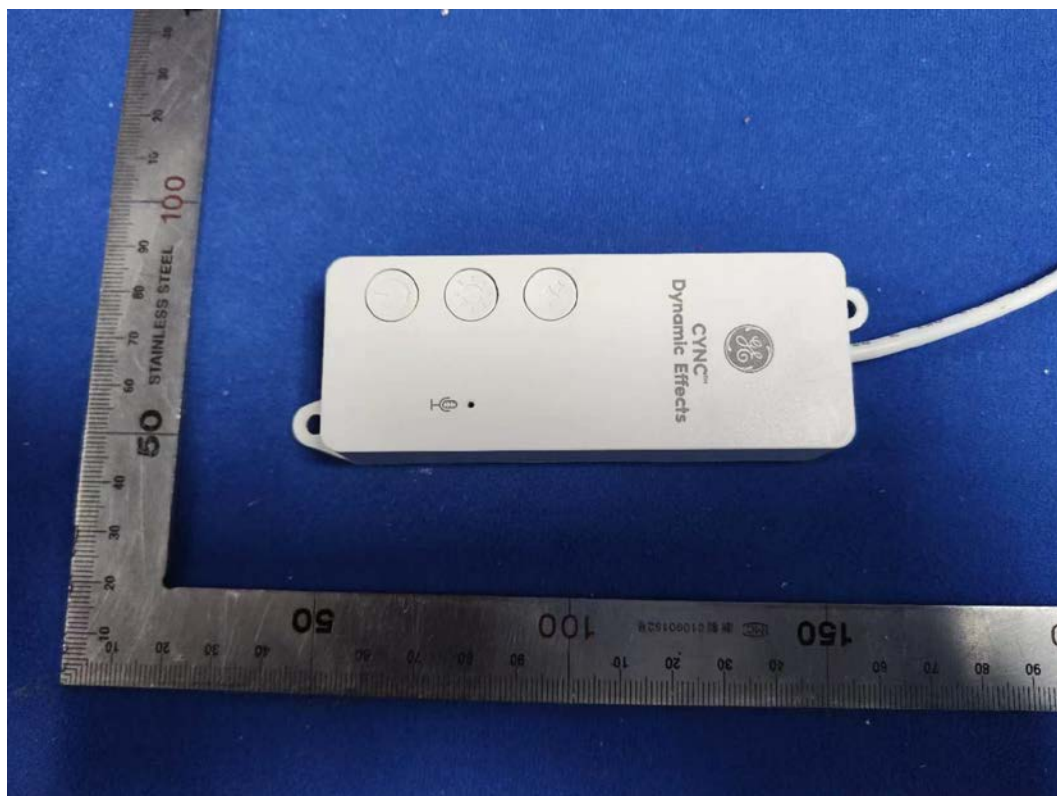
FIGURE 2 CYNCTILE (M/N: CFIXTIHCDEN) CONTROLLER TOP
