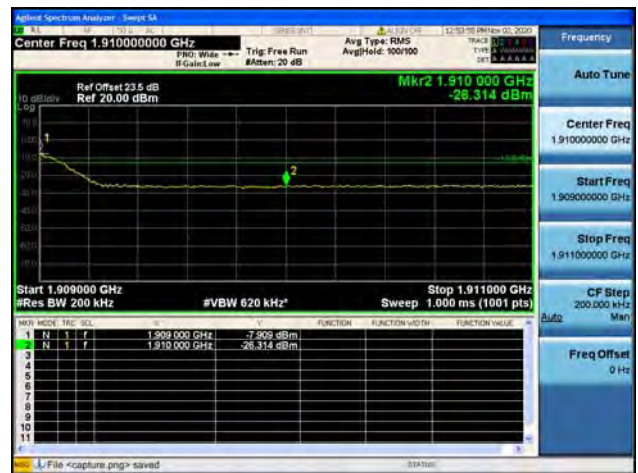
Band2 / 20MHz / High CH / QPSK / FULL RB
