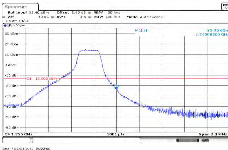
Band4-3MHz-16QAM-20385-15RB#0
