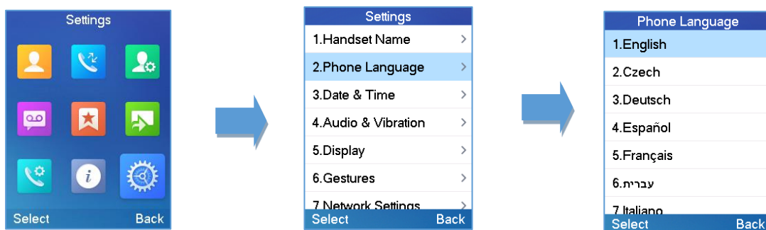
Figure 24: Handsets Language
