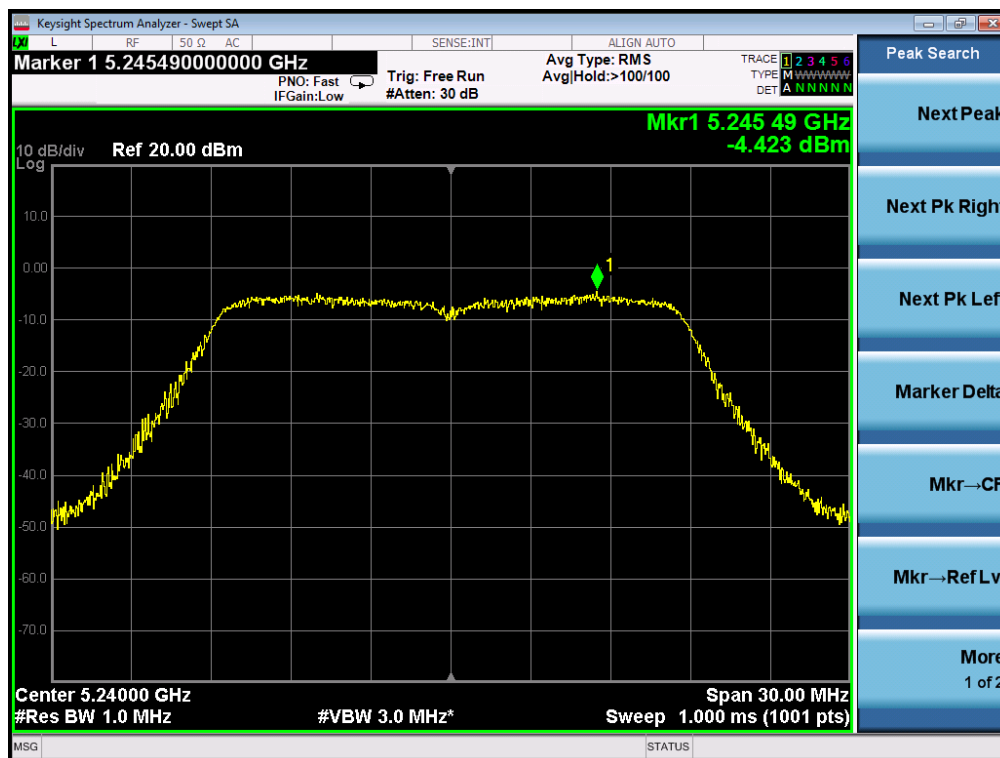
TEST PLOT OF SPECTRAL DENSITY FOR 5240MHz AT CHAIN 1
