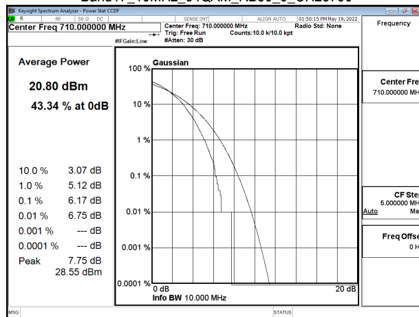
Band17_10MHz_64QAM_RB50_0_CH23800
