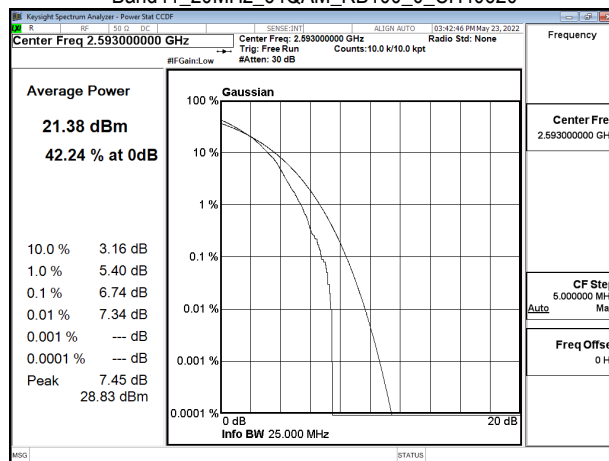
Band41_20MHz_64QAM_RB100_0_CH40620
