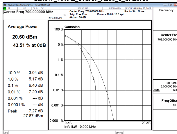
Band17_10MHz_64QAM_RB50_0_CH23790
