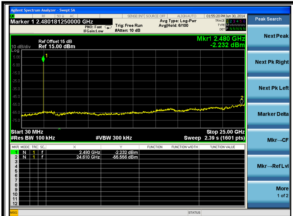
(Plot I.1: Channel = 78, 30MHz to 25GHz @ 8-DPSK)
