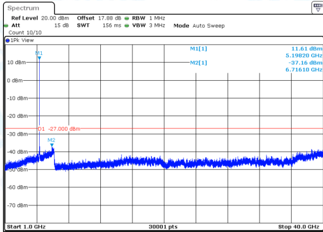
11A-CDD-Ant1-5200-1000~40000-PASS
