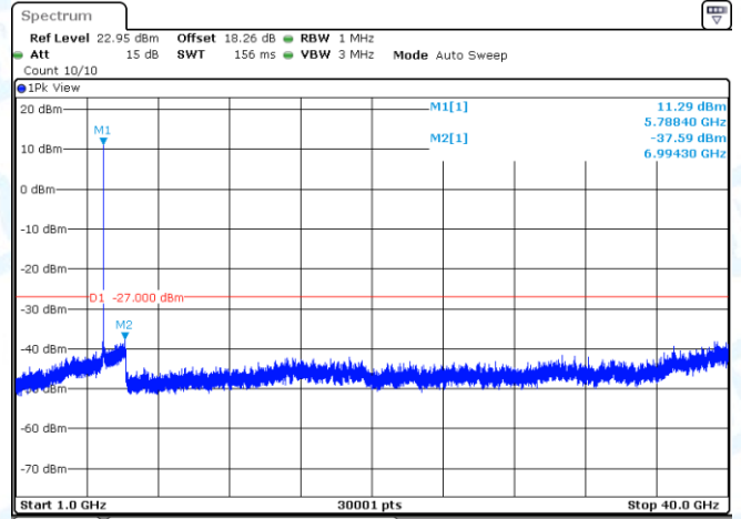
11N20MIMO-Ant2-5785-1000~40000-PASS
