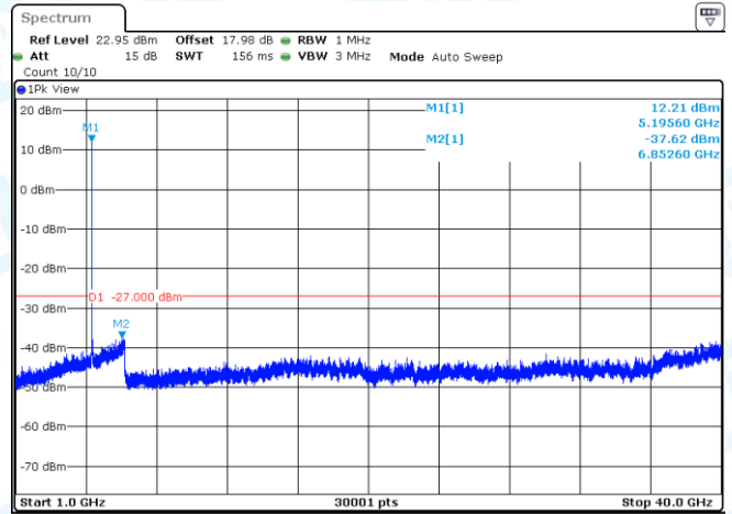
11A-CDD-Ant2-5200-1000~40000-PASS
