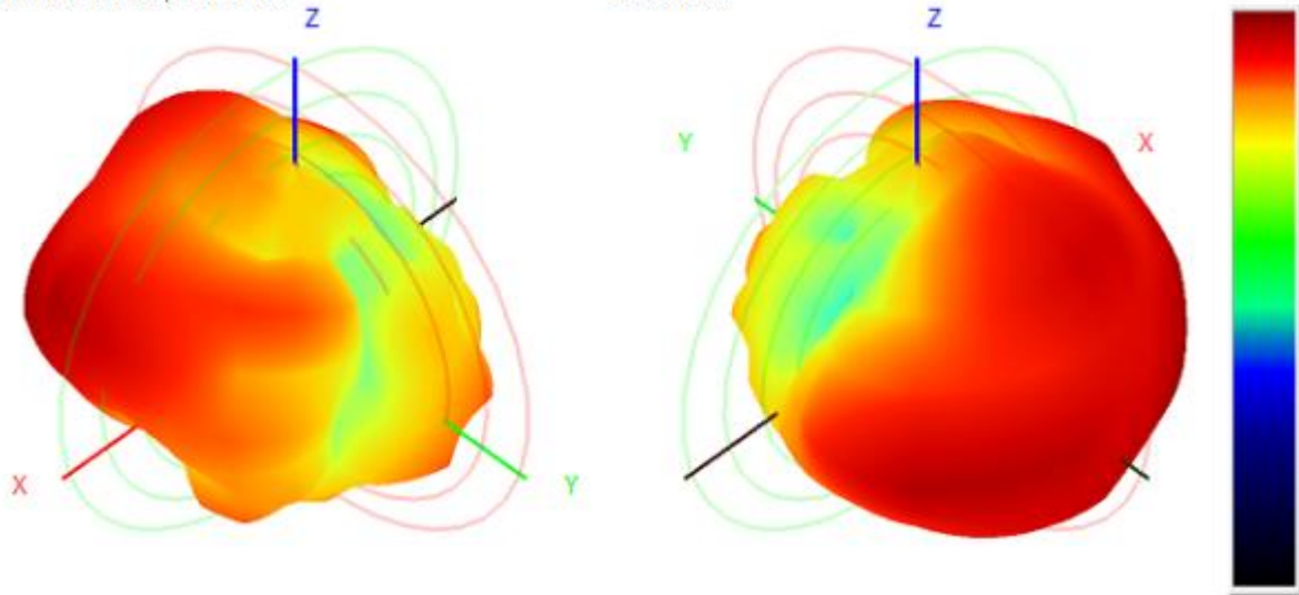
2490.0MHz H+V, Eff: 43.6%
