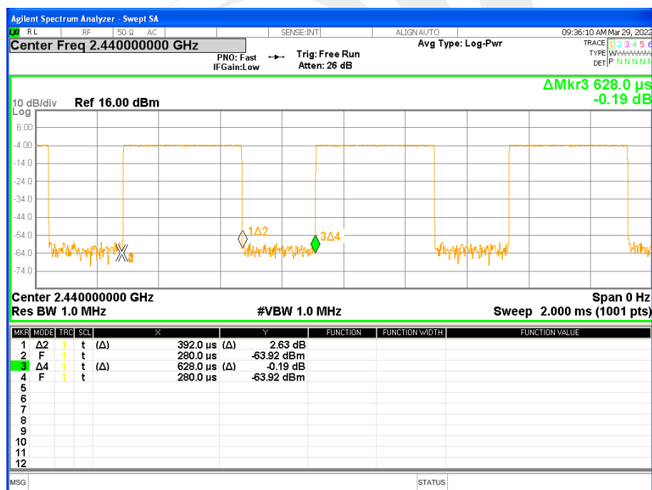
Duty cycle
