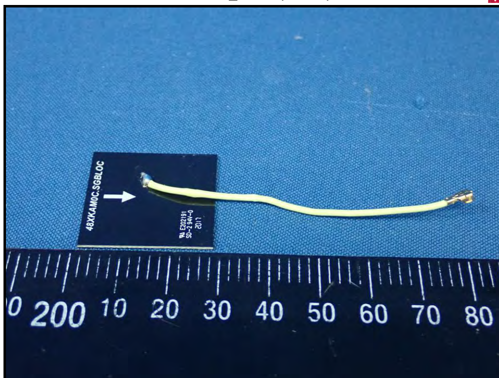
WiFi LB_1 Ant. (Dual A)
