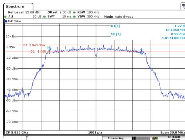
6dB BW_802.11a_5825MHz
