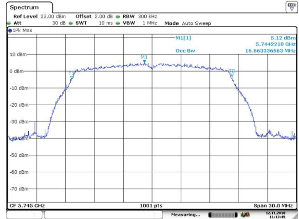
OBW_802.11a_5745MHz
