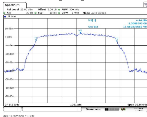
OBW_802.11a_5300MHz
