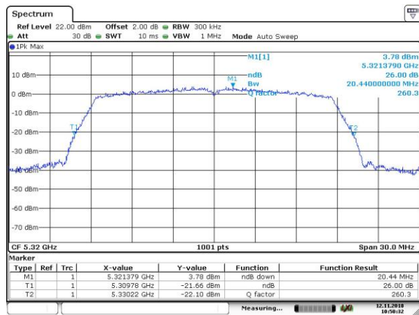
26dB_802.11n_HT20_5320MHz
