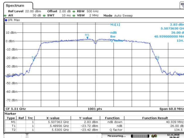
26dB_802.11n_HT40_5510MHz
