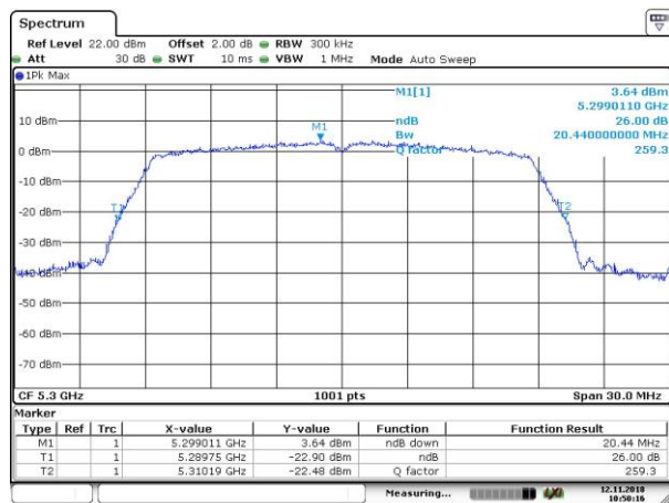
26dB_802.11n_HT20_5300MHz
