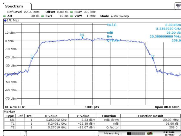
26dB_802.11n_HT20_5260MHz
