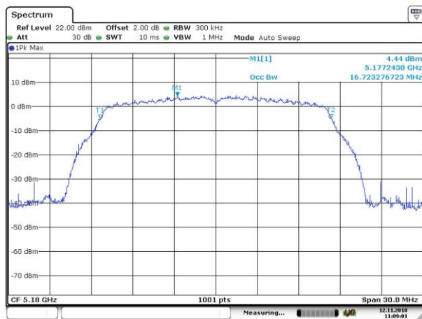
OBW_802.11a_5180MHz
