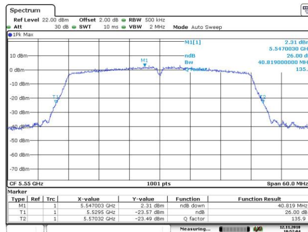
26dB_802.11n_HT40_5550MHz
