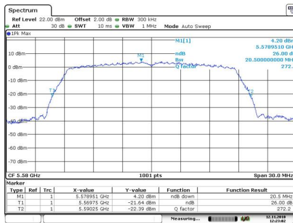
26dB_802.11n_HT20_5580MHz
