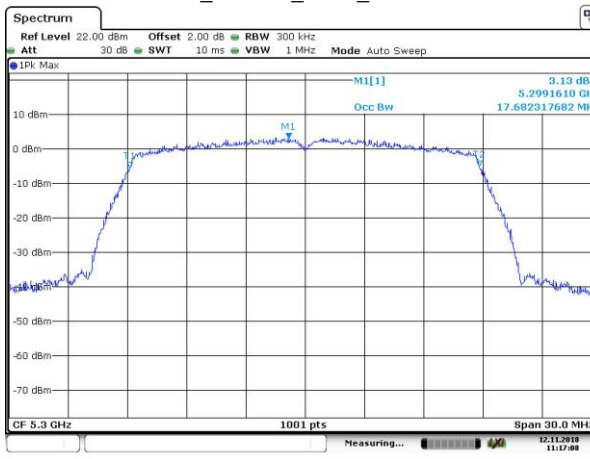
OBW_802.11n_HT20_5300MHz
