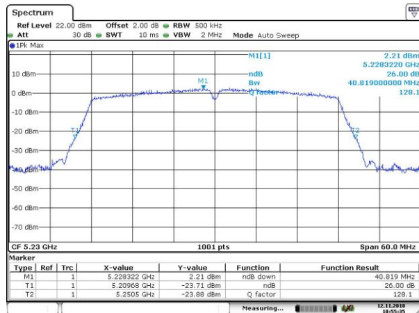
26dB_802.11n_HT40_5230MHz
