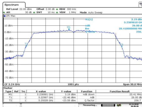
26dB_802.11n HT20_5240MHz
