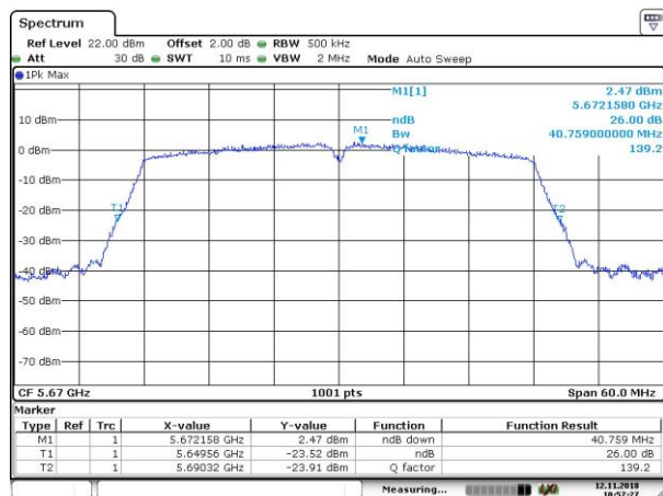
26dB_802.11n_HT40_5670MHz
