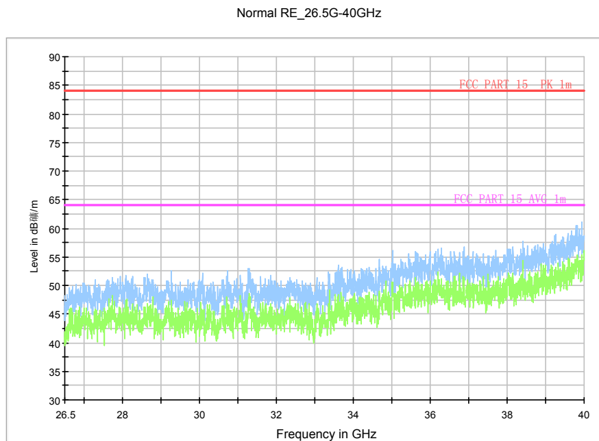
Fig. 68 Radiated Spurious Emission (802.11a, ch116, 26.5 GHz-40 GHz)
