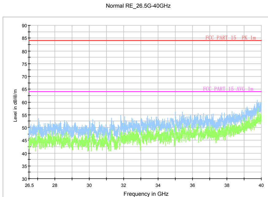
Fig. 50 Radiated Spurious Emission (802.11a, ch40, 26.5 GHz-40 GHz)
