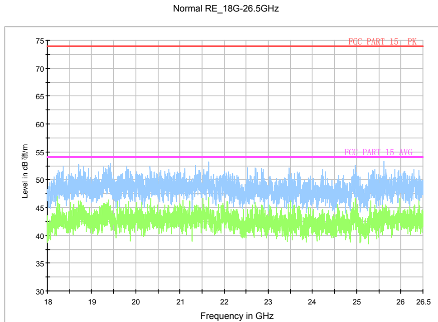
Fig. 49 Radiated Spurious Emission (802.11a, ch40, 18 GHz-26.5 GHz)
