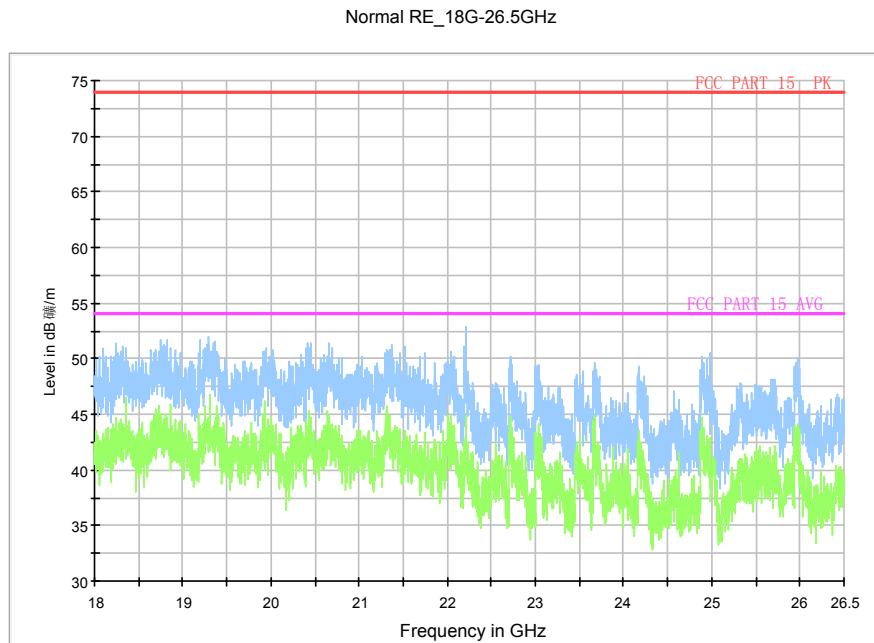
Fig. 67 Radiated Spurious Emission (802.11a, ch116, 18 GHz-26.5 GHz)
