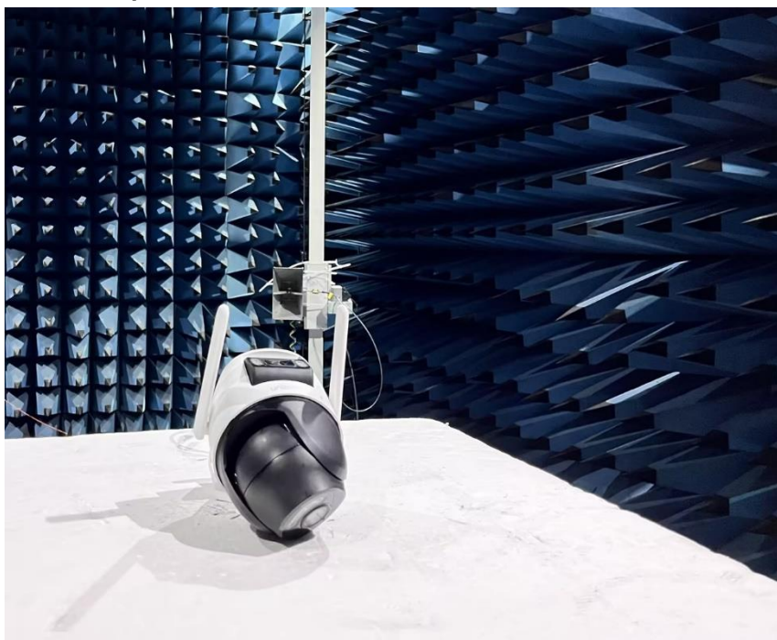
Radiated Spurious Emissions Above 1GHz
