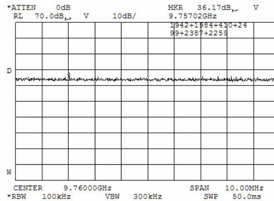
Plot 7.3.42 Radiated emission measurements at the forth harmonic of carrier frequency
