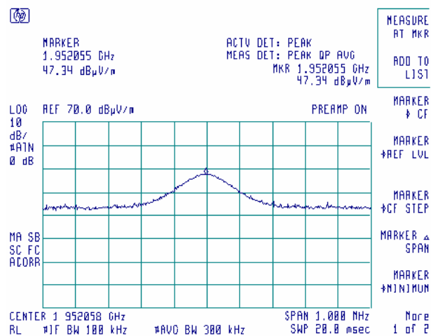
Plot 7.3.15 Radiated emission measurements at the 1952 MHz frequency
