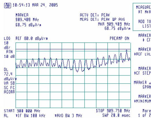
Plot 8.3.3 Emission mask test results at carrier frequency, right band edge
