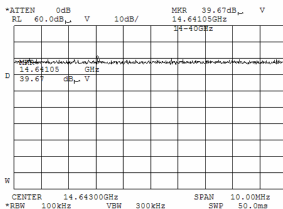
Plot 7.3.46 Radiated emission measurements at the sixth harmonic of carrier frequency
