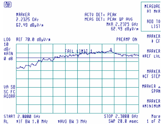
Plot 7.3.17 Radiated emission measurements from at 2236 MHz
