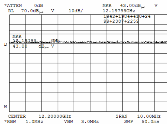
Plot 7.3.44 Radiated emission measurements at the fifth harmonic of carrier frequency
