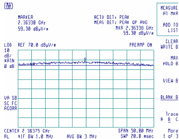
Plot 7.3.23 Radiated emission measurements at 2364 MHz
