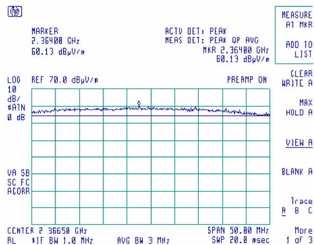
Plot 7.3.21 Radiated emission measurements at 2364 MHz
