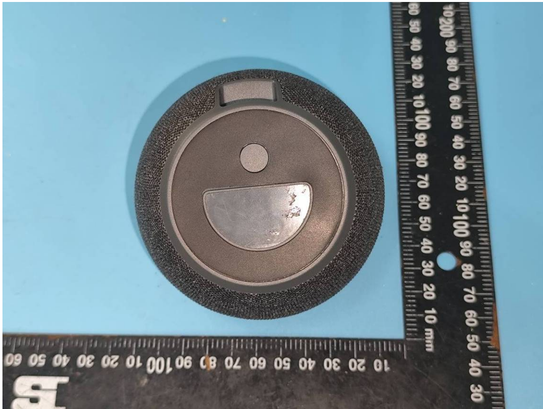
Type-C Port
