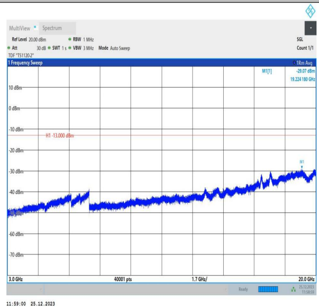
66-66-10MHz-5MHz-16QAM-16QAM-132572-132644-1RB#4 9-0RB#0-3000~20000MHz-PASS
