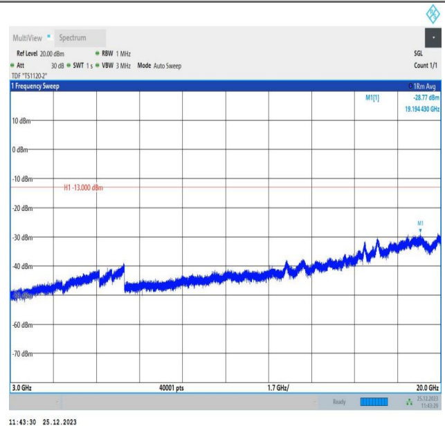
66-66-10MHz-5MHz-16QAM-16QAM-132022-132094-1RB#4 9-0RB#0-3000~20000MHz-PASS
