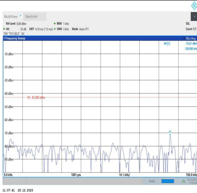
66-66-10MHz-5MHz-QPSK-QPSK-132572-132644-1RB#49-0RB#0-0.009~0.15MHz-PASS
