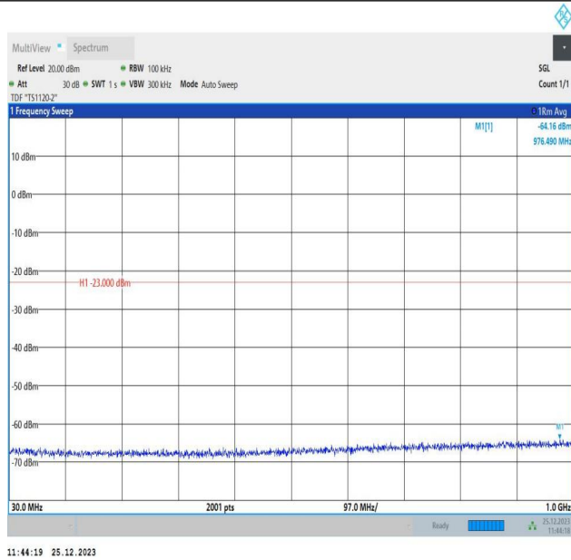
66-66-10MHz-5MHz-QPSK-QPSK-132022-132094-1RB#0-1 RB#24-30~1000MHz-PASS
