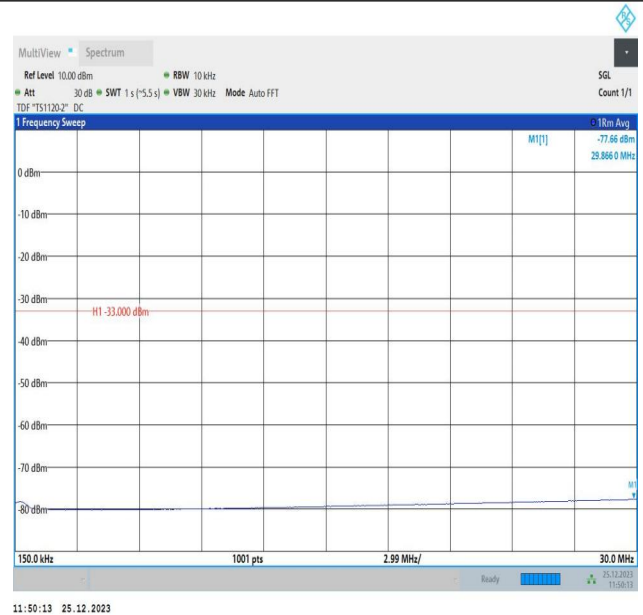
66-66-10MHz-5MHz-QPSK-QPSK-132397-132469-1RB#49-0RB#0-0.15~30MHz-PASS
