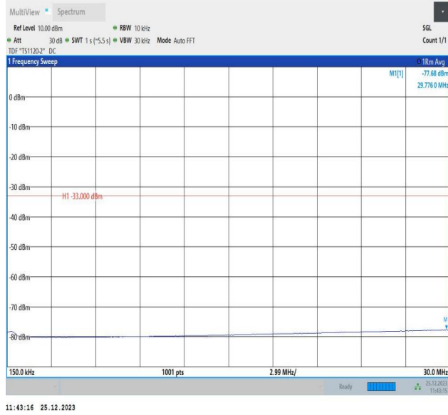
66-66-10MHz-5MHz-16QAM-16QAM-132022-132094-1RB#4 9-0RB#0-0.15~30MHz-PASS
