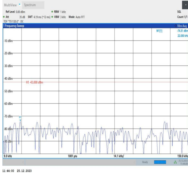
66-66-10MHz-5MHz-QPSK-QPSK-132022-132094-1RB#0-1 RB#24-0.009~0.15MHz-PASS
