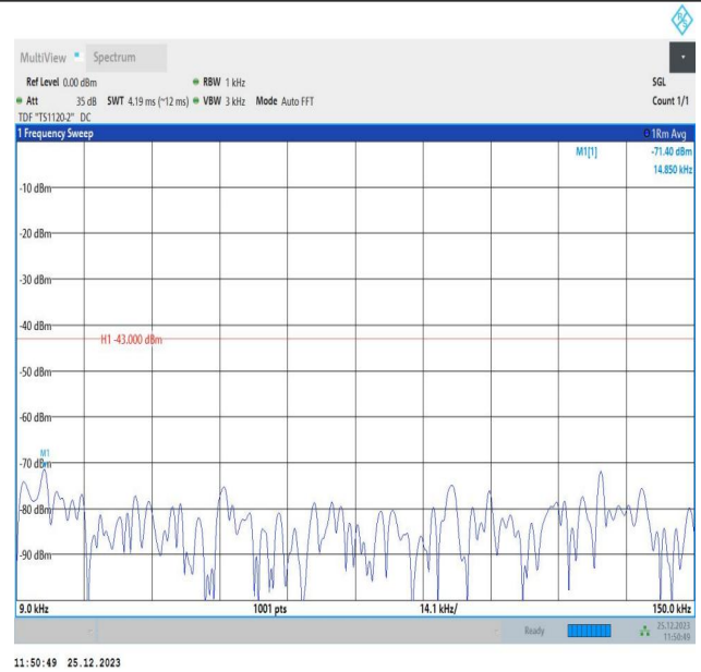
66-66-10MHz-5MHz-16QAM-16QAM-132397-132469-1RB#4 9-ORB#0-0.009~0.15MHz-PASS
