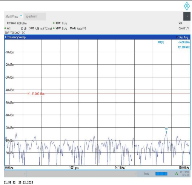
66-66-10MHz-5MHz-16QAM-16QAM-132572-132644-1RB#4 9-ORB#0-0.009~0.15MHz-PASS
