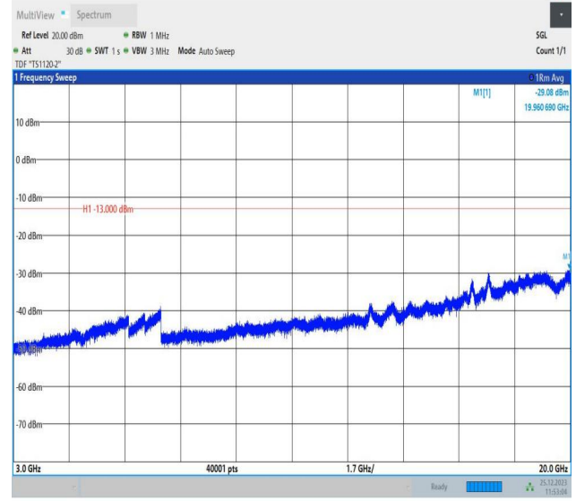
66-66-10MHz-5MHz-16QAM-16QAM-132397-132469-1RB#0-1RB#24-3000~20000MHz-PASS
