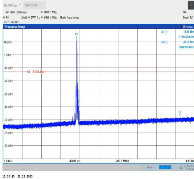
66-66-10MHz-5MHz-16QAM-16QAM-132572-132644-1RB#0-1RB#24-1000~3000MHz-PASS
