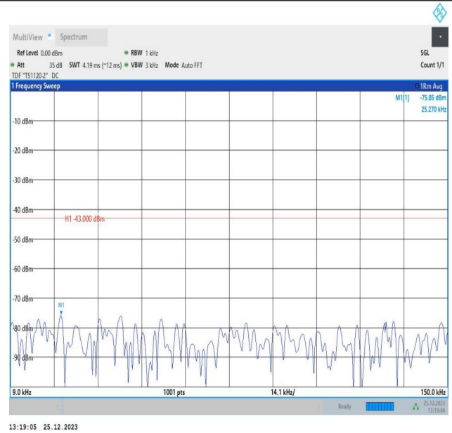
66-66-10MHz-10MHz-16QAM-16QAM-132022-132121-1RB# 49-ORB#0-0.009~0.15MHz-PASS
