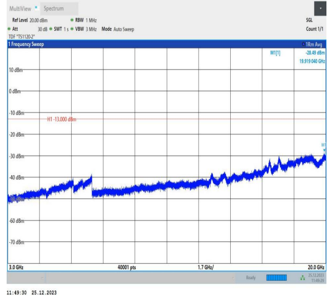
66-66-10MHz-5MHz-16QAM-16QAM-132397-132469-1RB#0-0RB#0-3000~20000MHz-PASS
