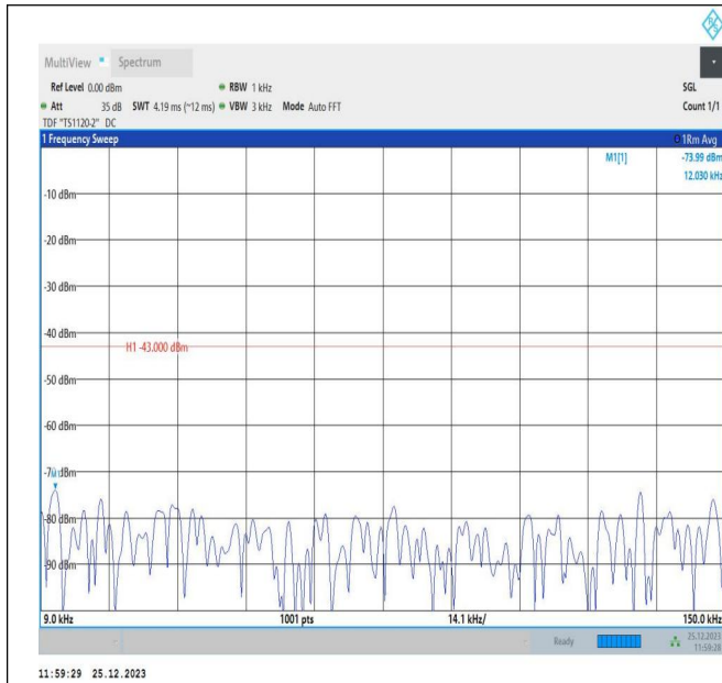
66-66-10MHz-5MHz-QPSK-QPSK-132572-132644-1RB#0-1 RB#24-0.009~0.15MHz-PASS
