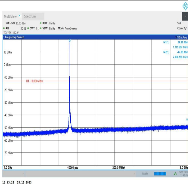
66-66-10MHz-5MHz-16QAM-16QAM-132022-132094-1RB#4 9-0RB#0-1000~3000MHz-PASS
