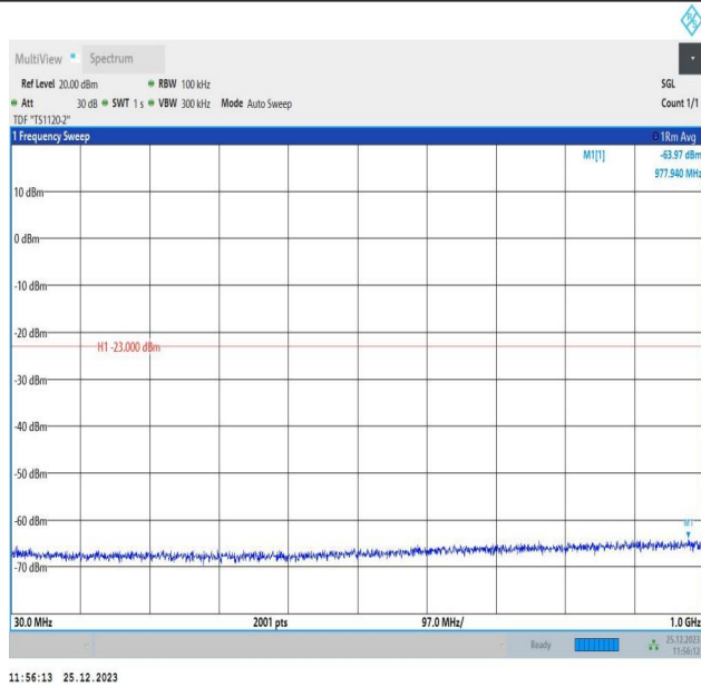
66-66-10MHz-5MHz-QPSK-QPSK-132572-132644-1RB#0-0 RB#0-30~1000MHz-PASS
