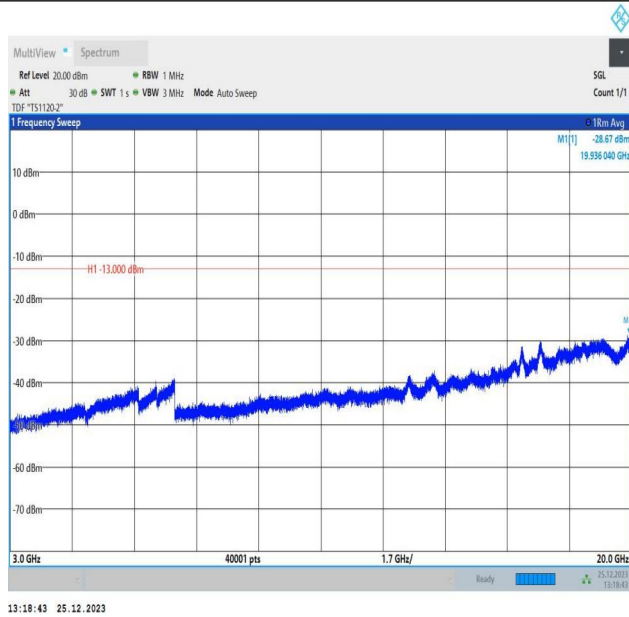
66-66-10MHz-10MHz-QPSK-QPSK-132022-132121-1RB#49 -ORB#0-3000~20000MHz-PASS
