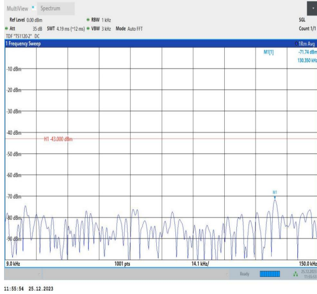
66-66-10MHz-5MHz-QPSK-QPSK-132572-132644-1RB#0-0 RB#0-0.009~0.15MHz-PASS
