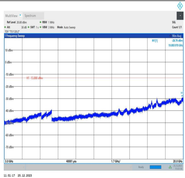
66-66-10MHz-5MHz-16QAM-16QAM-132397-132469-1RB#4 9-0RB#0-3000~20000MHz-PASS
