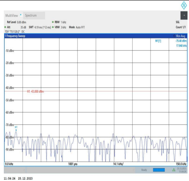
66-66-10MHz-5MHz-16QAM-16QAM-132397-132469-50RB#0-25RB#0-0.009~0.15MHz-PASS
