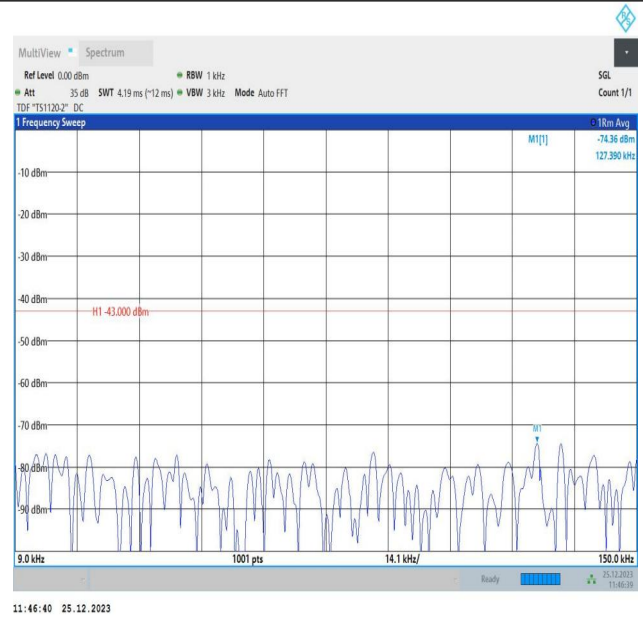
66-66-10MHz-5MHz-16QAM-16QAM-132022-132094-50RB#0-25RB#0-0.009~0.15MHz-PASS
