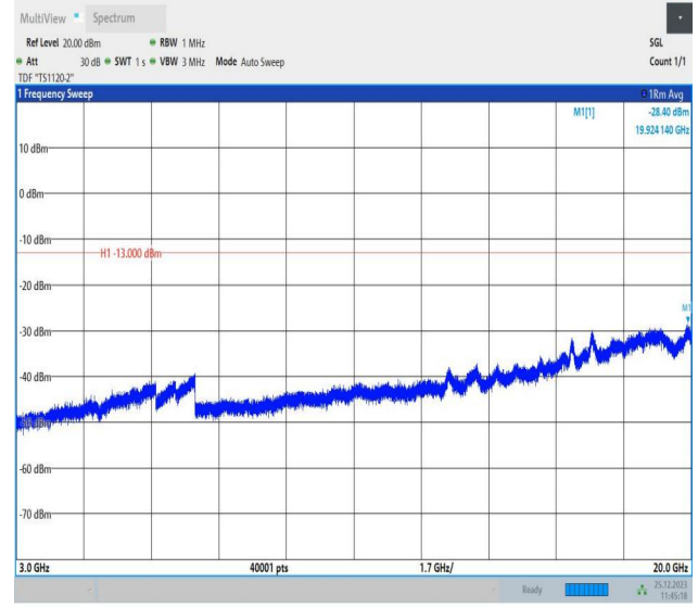
66-66-10MHz-5MHz-16QAM-16QAM-132022-132094-1RB#0-1RB#24-3000~20000MHz-PASS
