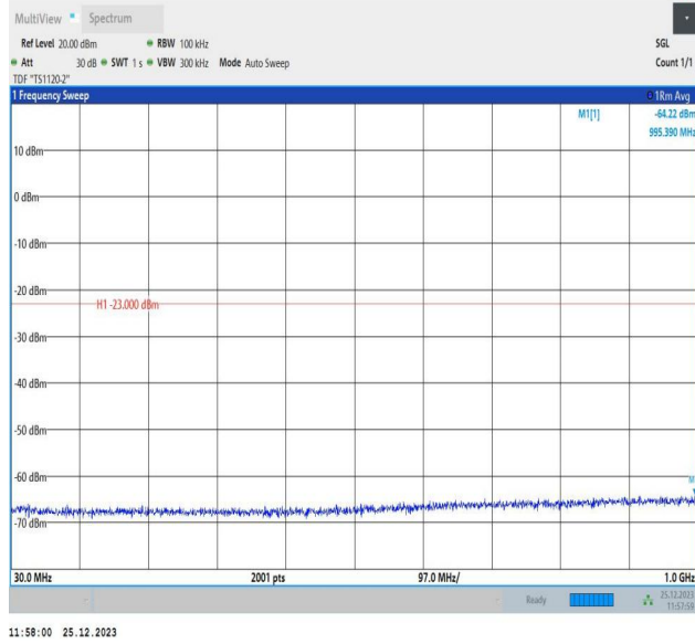
66-66-10MHz-5MHz-QPSK-QPSK-132572-132644-1RB#49- ORB#0-30~1000MHz-PASS
