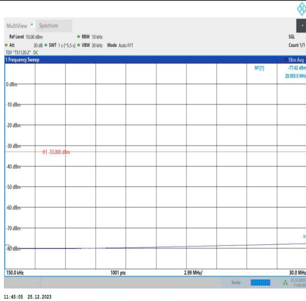
66-66-10MHz-5MHz-16QAM-16QAM-132022-132094-1RB#0 -1RB#24-0.15~30MHz-PASS
