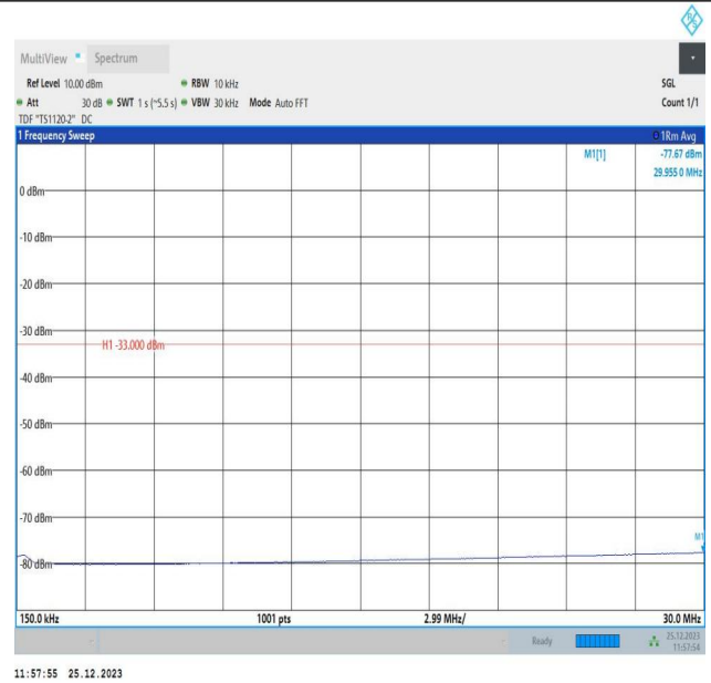
66-66-10MHz-5MHz-QPSK-QPSK-132572-132644-1RB#49-0RB#0-0.15~30MHz-PASS
