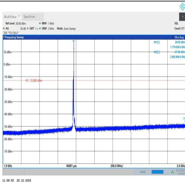
66-66-10MHz-5MHz-16QAM-16QAM-132572-132644-1RB#4 9-0RB#0-1000~3000MHz-PASS
