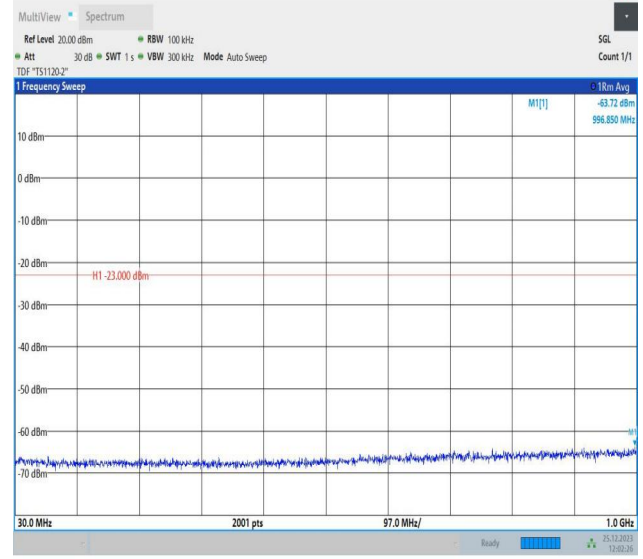
66-66-10MHz-5MHz-16QAM-16QAM-132572-132644-50RB# 0-25RB#0-30~1000MHz-PASS
