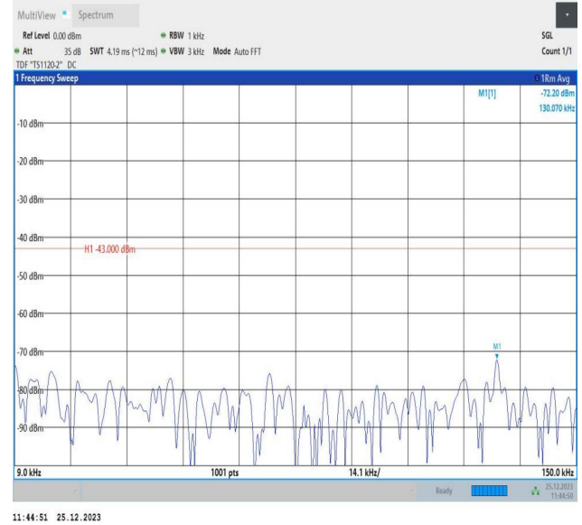
66-66-10MHz-5MHz-16QAM-16QAM-132022-132094-1RB#0- 1RB#24-0.009~0.15MHz-PASS
