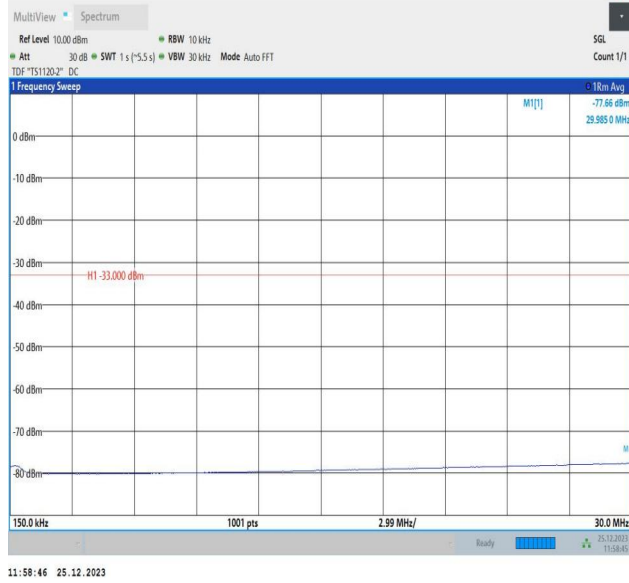
66-66-10MHz-5MHz-16QAM-16QAM-132572-132644-1RB#4 9-0RB#0-0.15~30MHz-PASS
