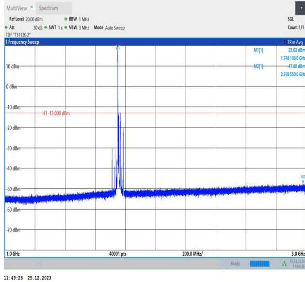
66-66-10MHz-5MHz-16QAM-16QAM-132397-132469-1RB#0-0RB#0-1000~3000MHz-PASS
