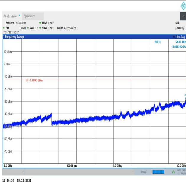
66-66-10MHz-5MHz-QPSK-QPSK-132572-132644-1RB#49- ORB#0-3000~20000MHz-PASS
