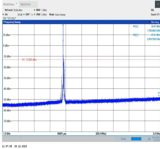
66-66-10MHz-5MHz-16QAM-16QAM-132572-132644-1RB#0-0RB#0-1000~3000MHz-PASS
