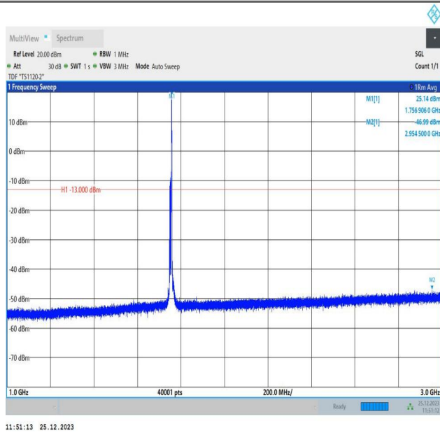
66-66-10MHz-5MHz-16QAM-16QAM-132397-132469-1RB#4 9-0RB#0-1000~3000MHz-PASS
