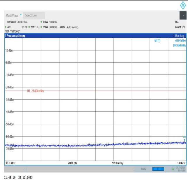
66-66-10MHz-5MHz-16QAM-16QAM-132022-132094-1RB#0- 1RB#24-30~1000MHz-PASS
