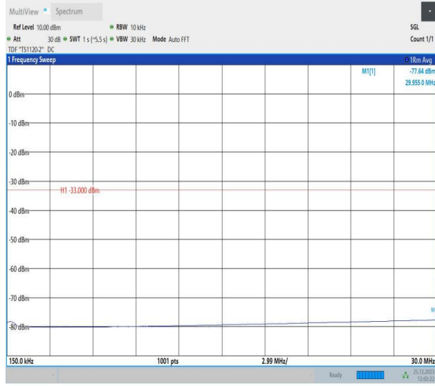
66-66-10MHz-5MHz-16QAM-16QAM-132572-132644-50RB# 0-25RB#0-0.15~30MHz-PASS
