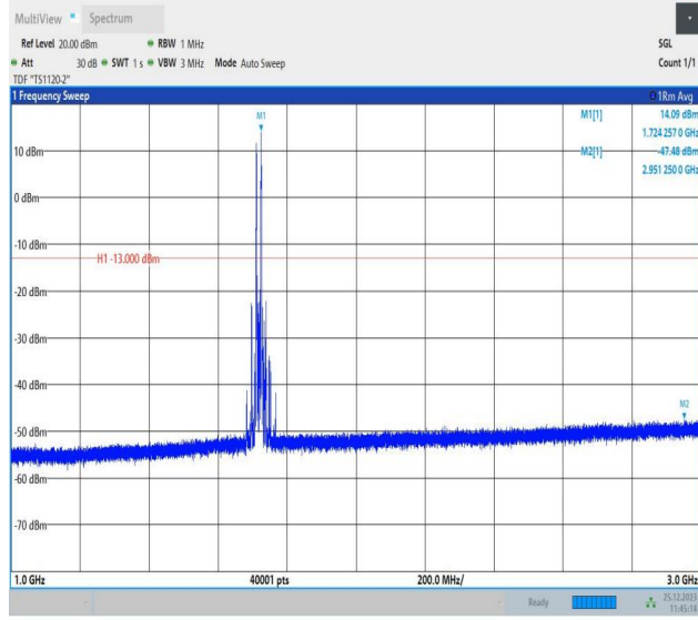
66-66-10MHz-5MHz-16QAM-16QAM-132022-132094-1RB#0-1RB#24-1000~3000MHz-PASS
