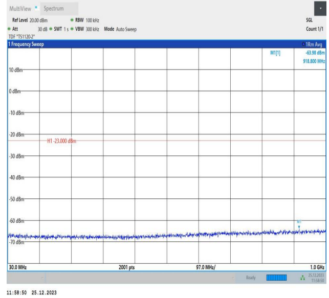
66-66-10MHz-5MHz-16QAM-16QAM-132572-132644-1RB#4 9-0RB#0-30~1000MHz-PASS
