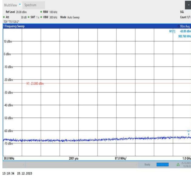
66-66-10MHz-10MHz-QPSK-QPSK-132022-132121-1RB#49 -ORB#0-30~1000MHz-PASS
