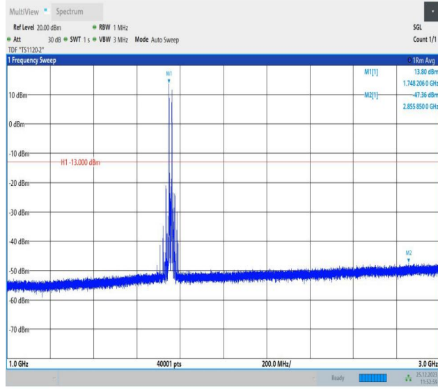
66-66-10MHz-5MHz-16QAM-16QAM-132397-132469-1RB#0-1RB#24-1000~3000MHz-PASS
