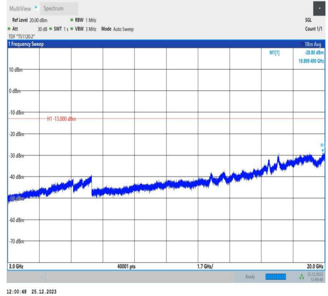
66-66-10MHz-5MHz-16QAM-16QAM-132572-132644-1RB#0-1RB#24-3000~20000MHz-PASS
