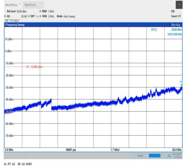
66-66-10MHz-5MHz-16QAM-16QAM-132572-132644-1RB#0-0RB#0-3000~20000MHz-PASS
