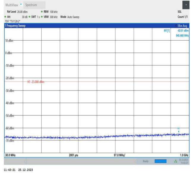
66-66-10MHz-5MHz-16QAM-16QAM-132022-132094-1RB#4 9-0RB#0-30~1000MHz-PASS
