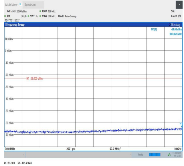
66-66-10MHz-5MHz-16QAM-16QAM-132397-132469-1RB#4 9-0RB#0-30~1000MHz-PASS
