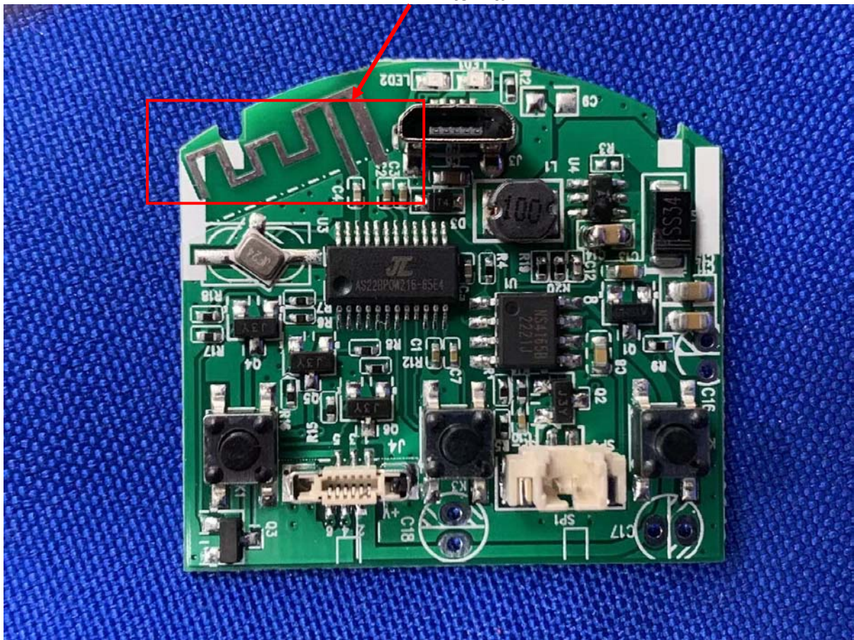
BT Antenna
