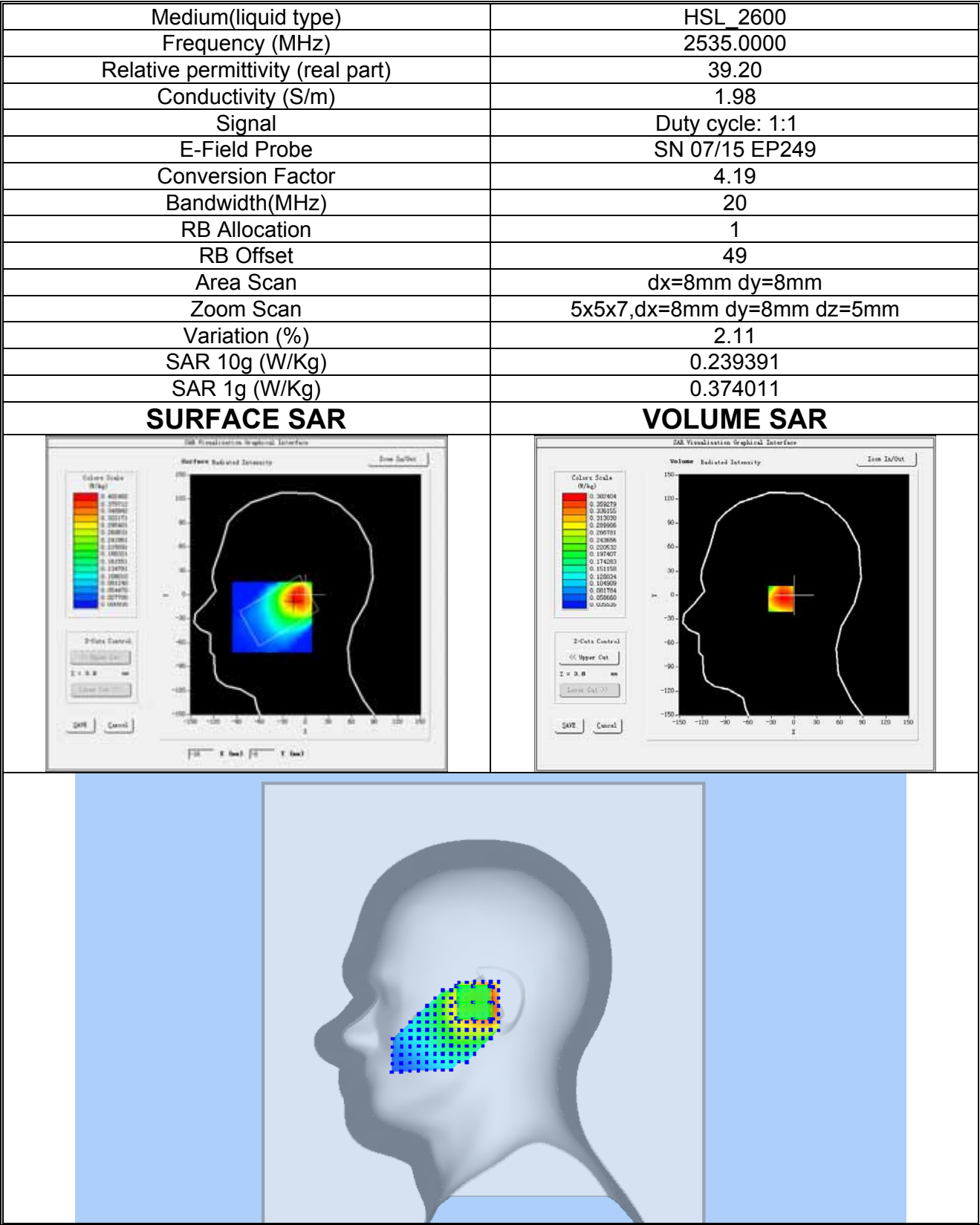
Plot 19:LTE BAND7, Middle channel (Right Head Cheek) Product Description: Smart phone Test Date: 2017-12-14
