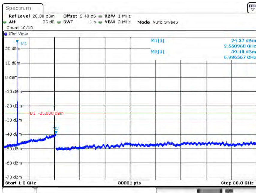
Band7-20MHz-16QAM-21350-1RB#0-Range2:1000~30000MHz
