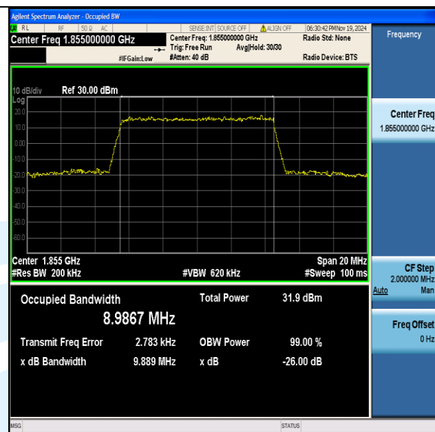
Band2-10MHz-16QAM-18650-50RB#0-PASS
