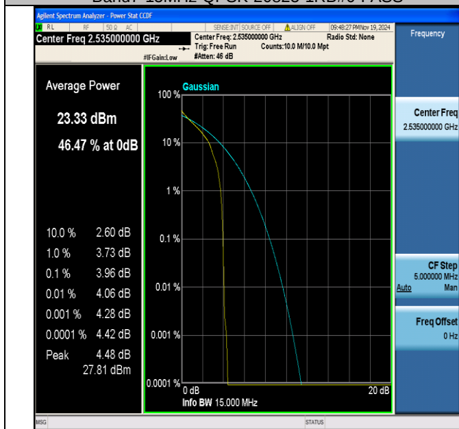
Band7-15MHz-QPSK-21100-1RB#0-PASS
