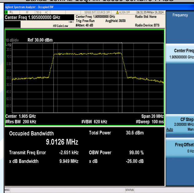
Band2-10MHz-16QAM-19150-50RB#0-PASS
