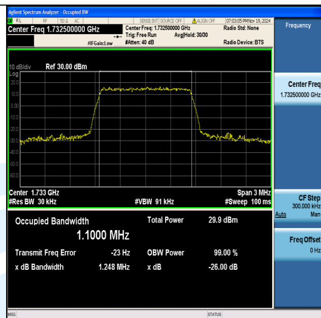
Band4-1.4MHz-QPSK-20175-6RB#0-PASS
