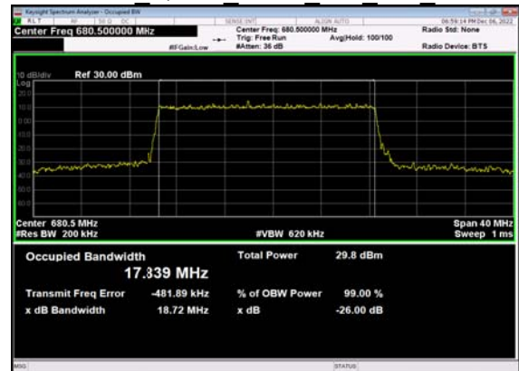
N71(20M)_DFT-s-OFDM_QPSK Outer Full Mid CH
