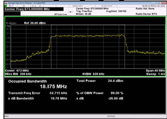
N71(20M)_CP-OFDM_256 QAM Outer Full Low CH
