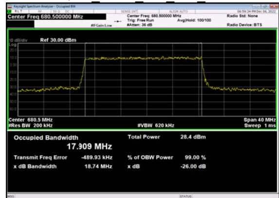
N71(20M)_DFT-s-OFDM_64 QAM Outer Full Mid CH
