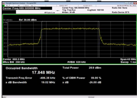
N71(20M)_DFT-s-OFDM_16 QAM Outer Full Mid CH
