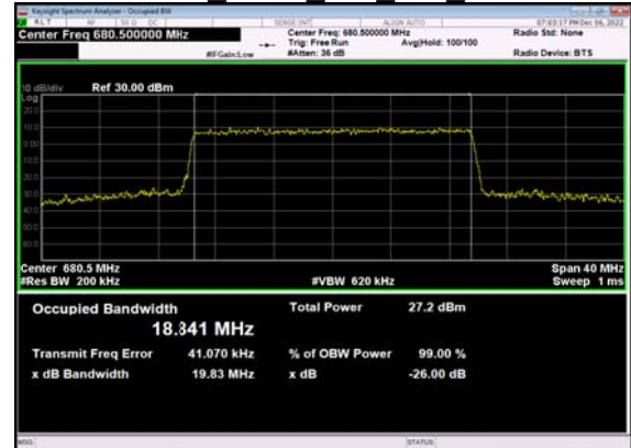
N71(20M)_CP-OFDM_64 QAM Outer Full Mid CH
