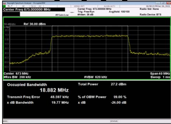
N71(20M)_CP-OFDM_64 QAM Outer Full Low CH
