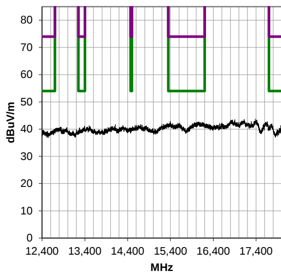
12400-18000 MHz, Run 22
