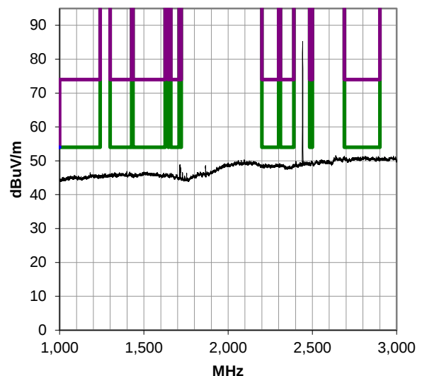
1000-3000 MHz, Run 19
