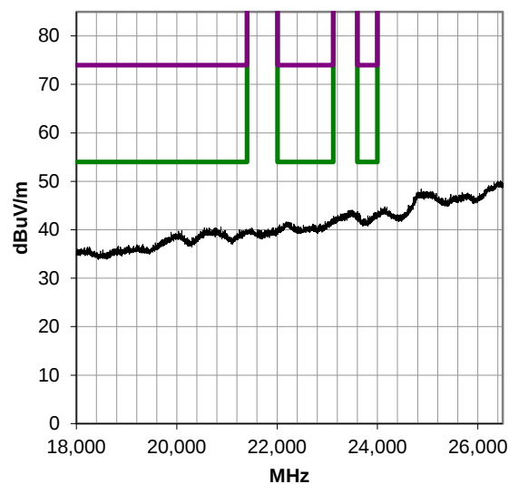
18000-26500 MHz, Run 34
