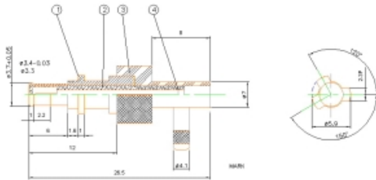
OCX 90 degree crimp connector
