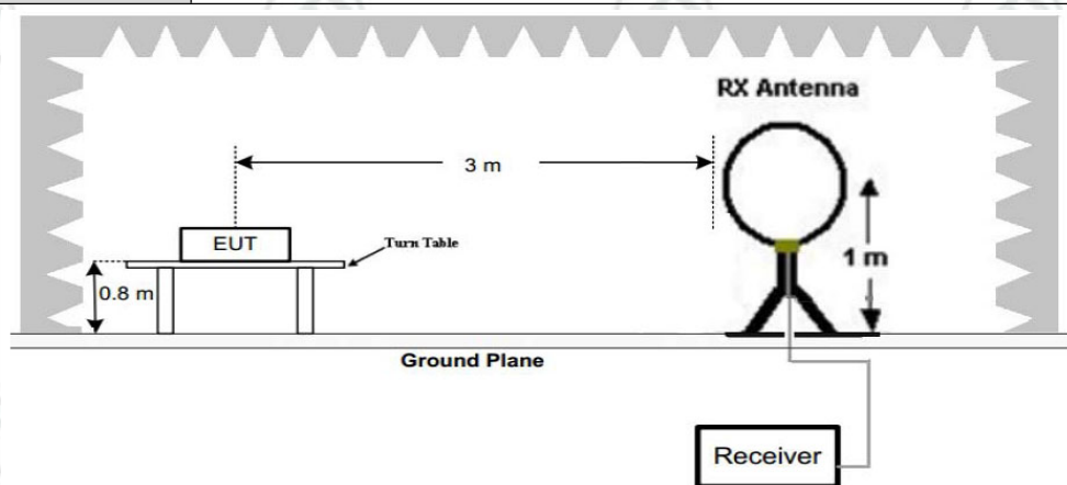
Figure 1. Below 30MHz
