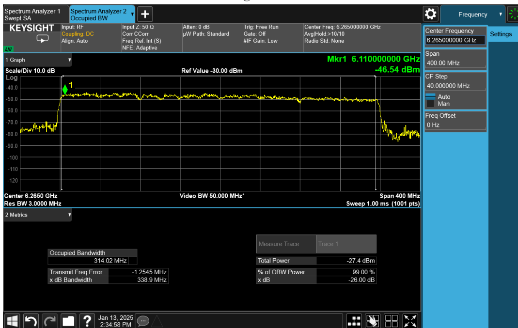
Plot 8: EUT 320MHz Bandwidth
