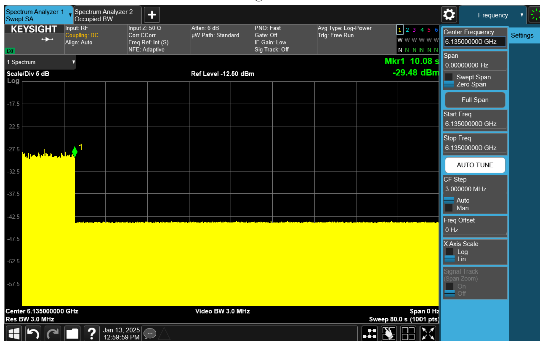
Plot 2: AWGN Signal Detection 20MHz
