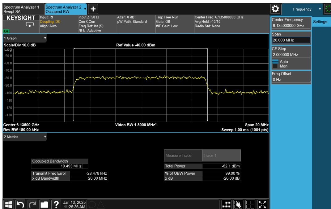
Plot 1: AWGN Signal BW/Power Details
