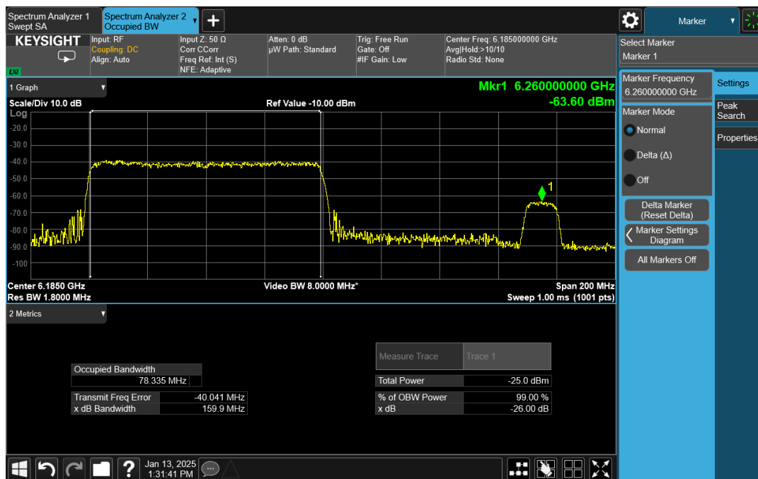
Plot 4: EUT 160MHz Bandwidth Reduction
