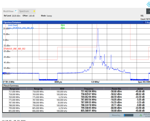
Band14-5MHz-QPSK-23305-25RB#0
