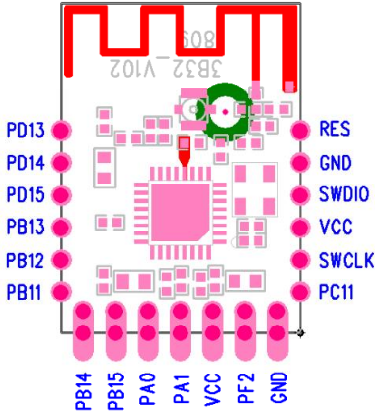
Figure 1 Pin Definition
