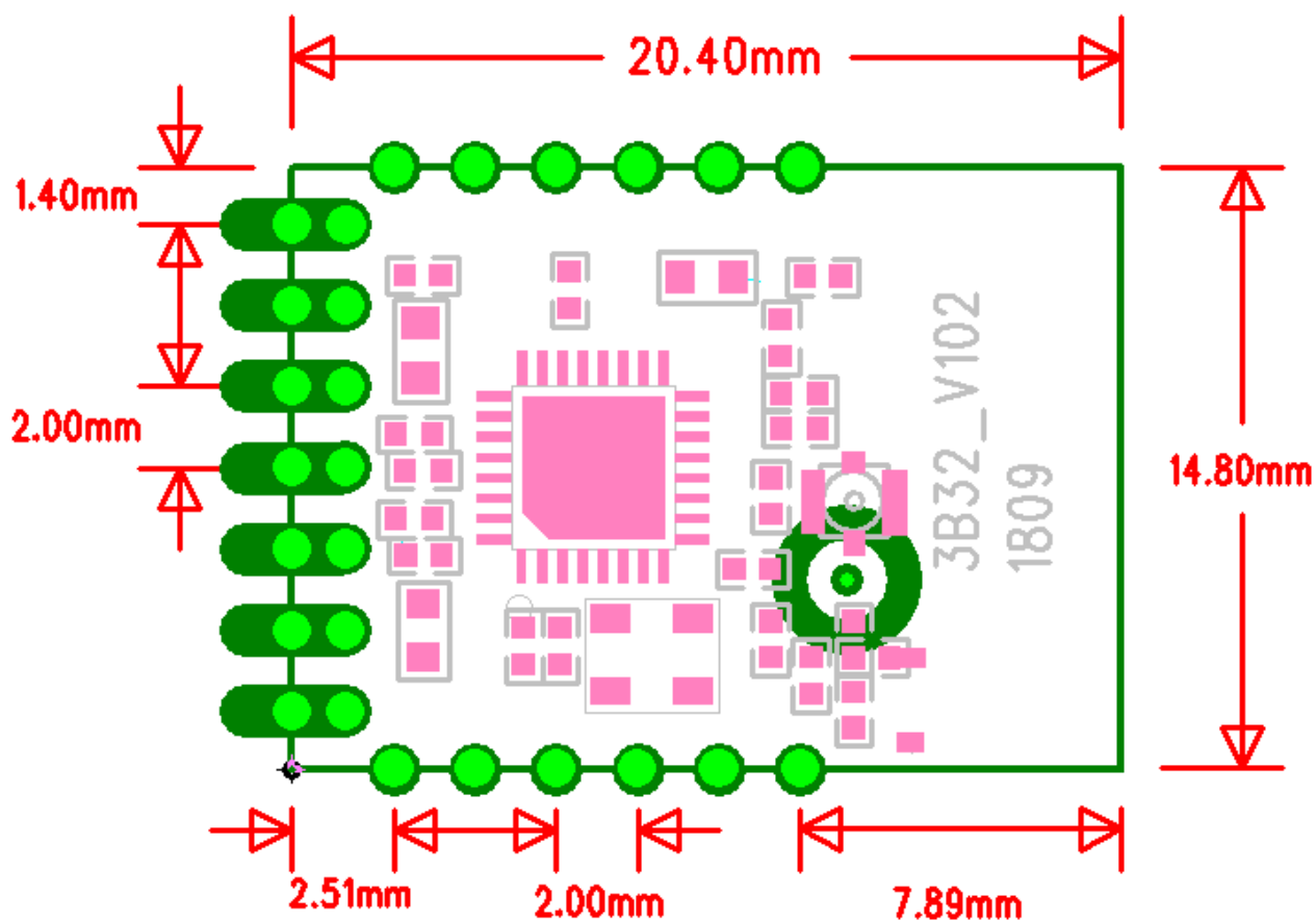
Figure 2 Module Size
