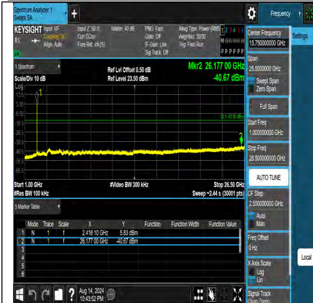
11g-CDD-Ant1-2412-1000~26500-PASS
