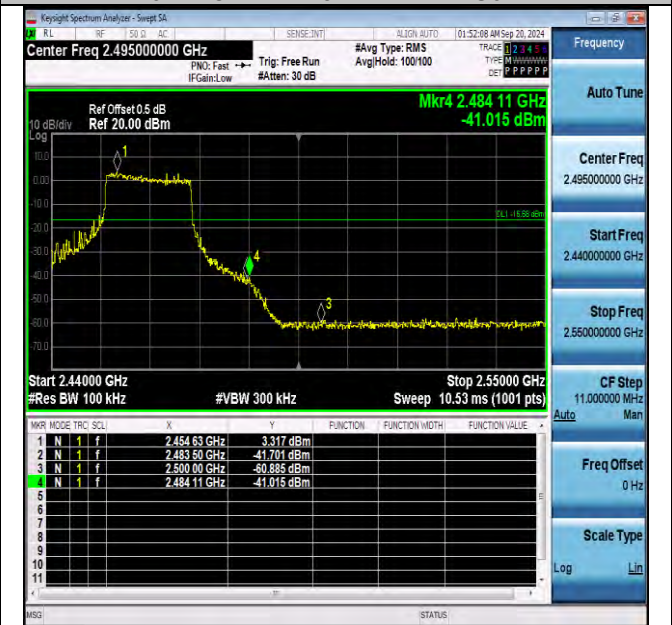
11be40MIMO-Ant2-2452-242Tone-RU62-PASS
