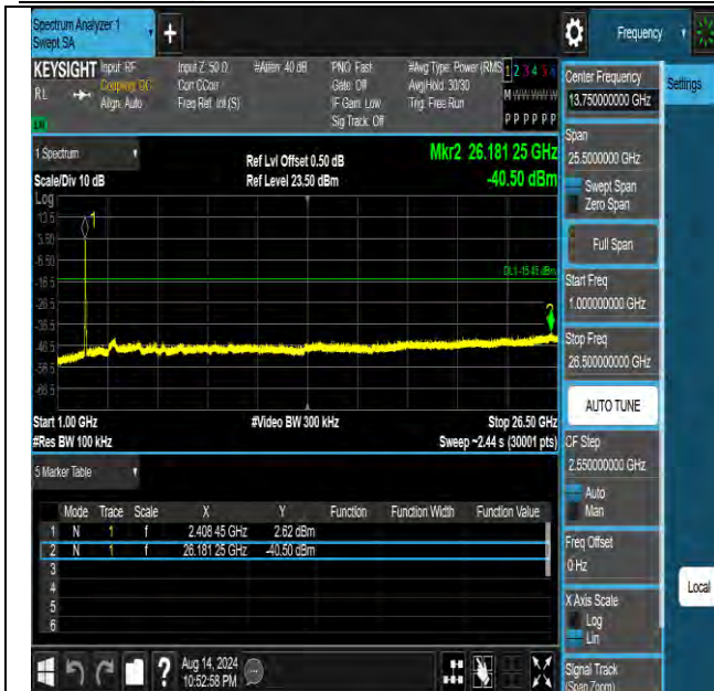
11n40MIMO-Ant1-2422-1000~26500-PASS
