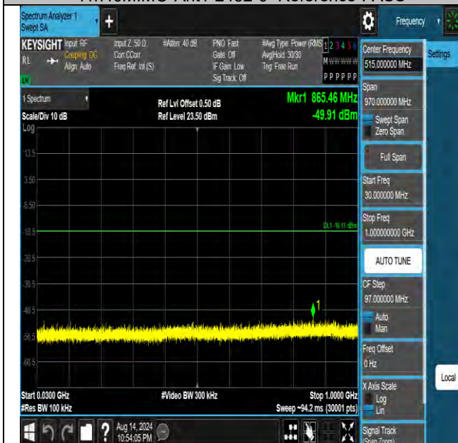
11n40MIMO-Ant1-2452-30~1000-PASS
