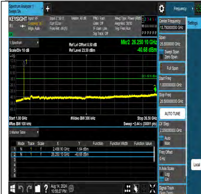
11n40MIMO-Ant1-2452-1000~26500-PASS
