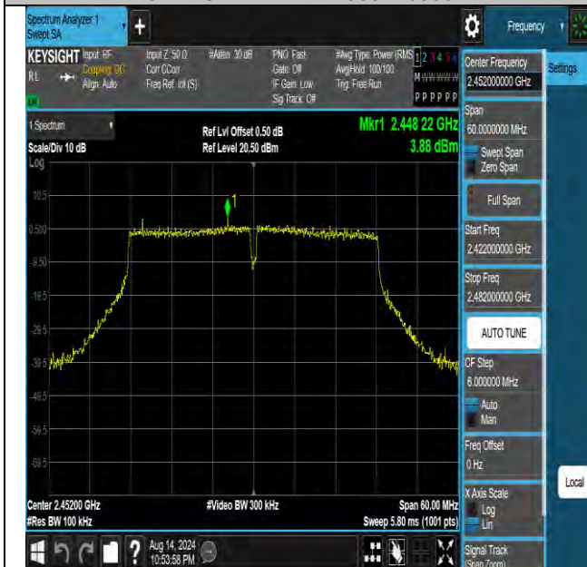
11n40MIMO-Ant1-2452-0~Reference-PASS
